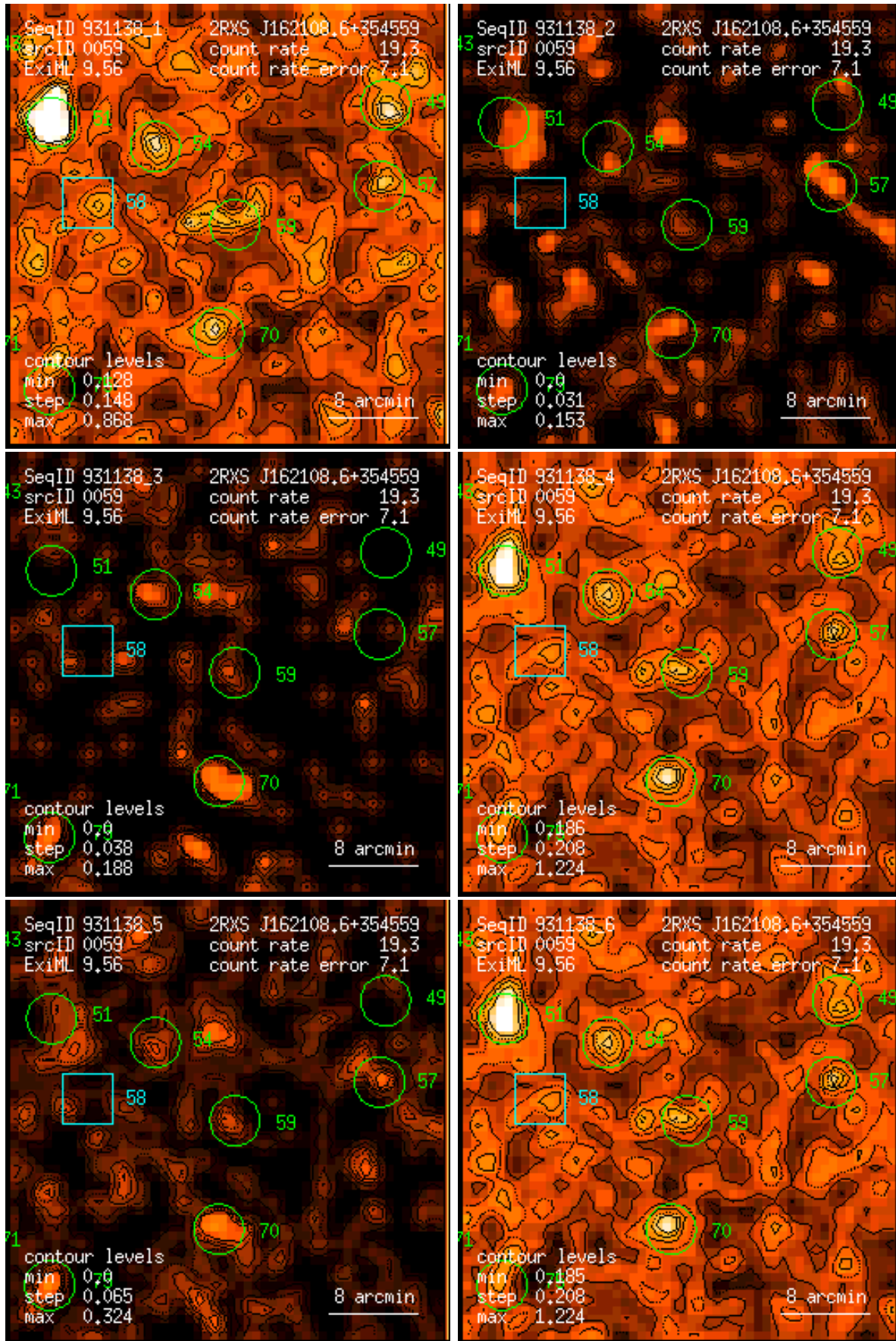
Figure 59: RASS 931138: detection 0059: band rate images, Gaussian filter: (1) PSPC channels 11 – 41, (2) 52 – 90, (3) 91 – 201, (4) 11 – 235, (5) 52 – 201, (6) 11 – 201. Broad band rates in counts/ks. Band rate contour levels in counts/ks/arcmin 2 .
