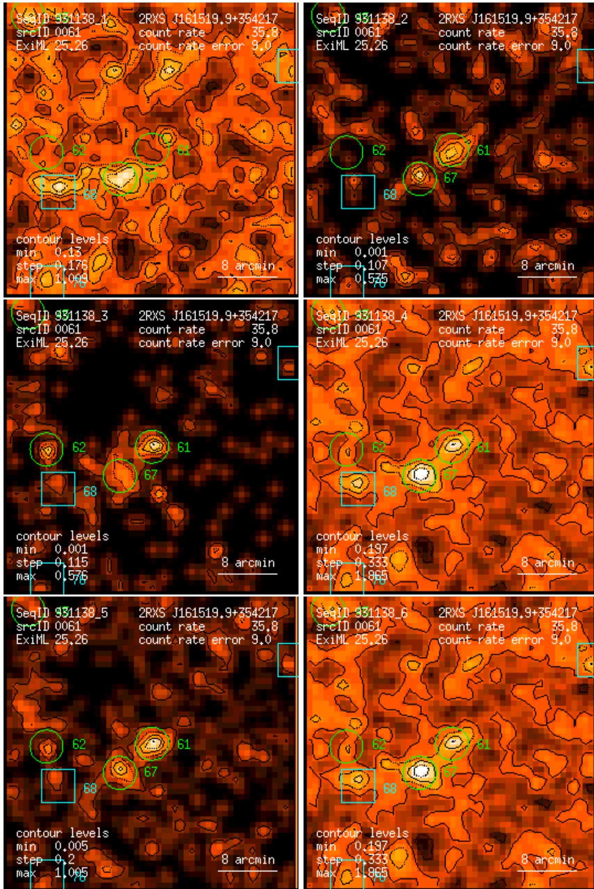
Figure 61: RASS 931138: detection 0061: band rate images, Gaussian filter: (1) PSPC channels 11 – 41, (2) 52 – 90, (3) 91 – 201, (4) 11 – 235, (5) 52 – 201, (6) 11 – 201. Broad band rates in counts/ks. Band rate contour levels in counts/ks/arcmin 2 .
