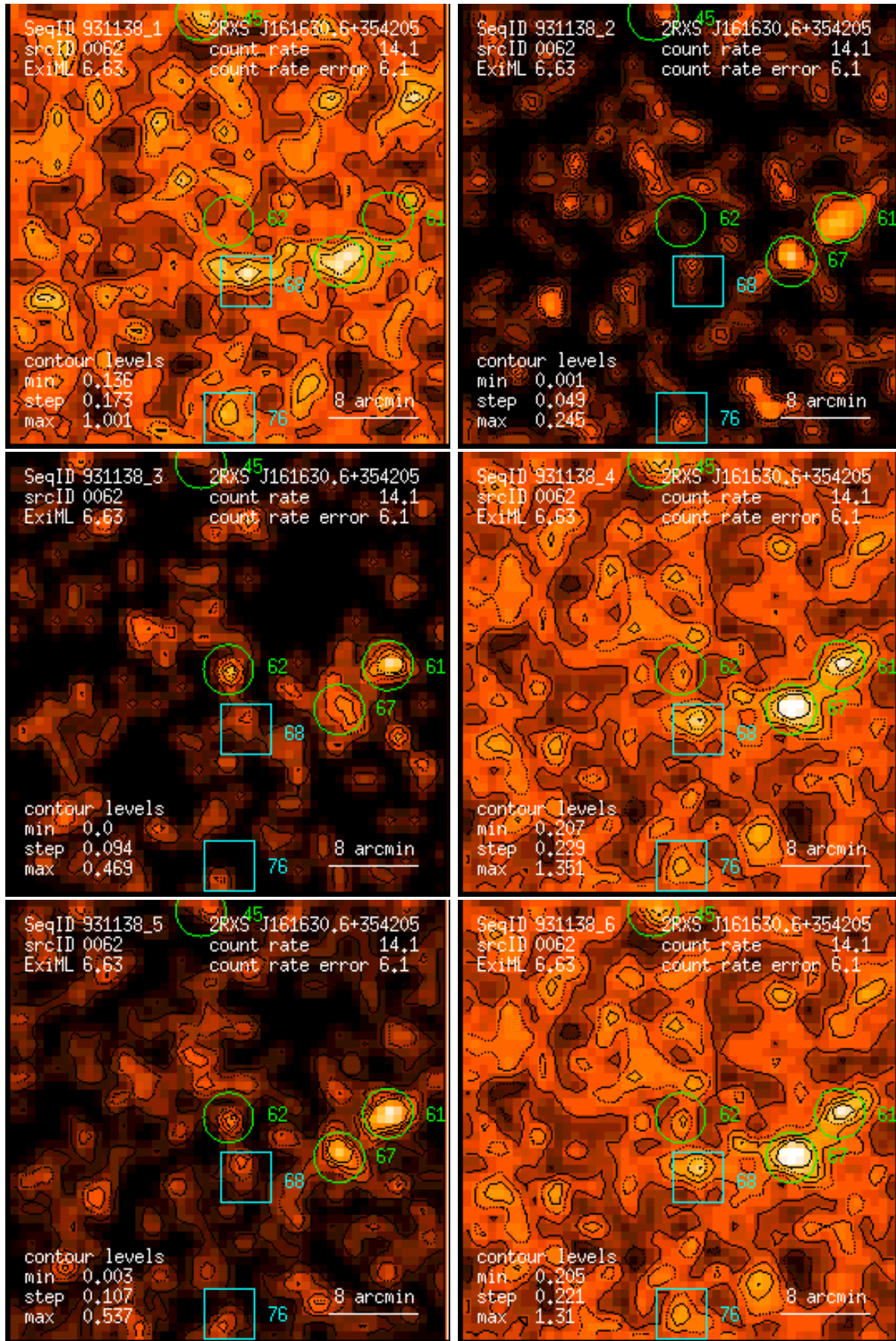
Figure 62: RASS 931138: detection 0062: band rate images, Gaussian filter: (1) PSPC channels 11 – 41, (2) 52 – 90, (3) 91 – 201, (4) 11 – 235, (5) 52 – 201, (6) 11 – 201. Broad band rates in counts/ks. Band rate contour levels in counts/ks/arcmin 2 .
