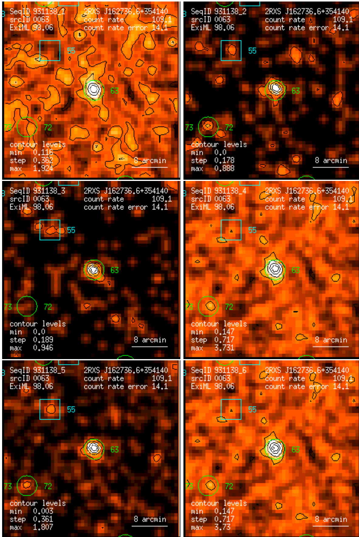
Figure 63: RASS 931138: detection 0063: band rate images, Gaussian filter: (1) PSPC channels 11 – 41, (2) 52 – 90, (3) 91 – 201, (4) 11 – 235, (5) 52 – 201, (6) 11 – 201. Broad band rates in counts/ks. Band rate contour levels in counts/ks/arcmin 2 .
