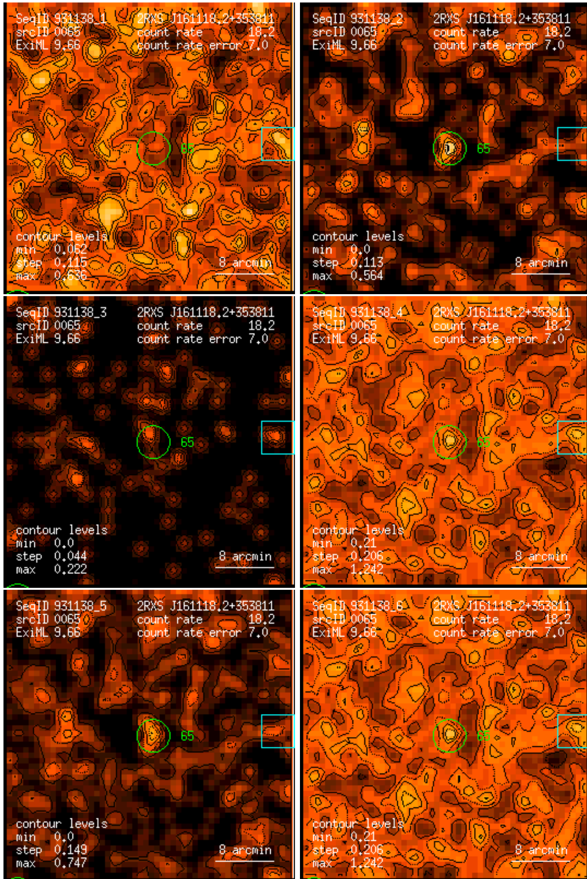
Figure 65: RASS 931138: detection 0065: band rate images, Gaussian filter: (1) PSPC channels 11 – 41, (2) 52 – 90, (3) 91 – 201, (4) 11 – 235, (5) 52 – 201, (6) 11 – 201. Broad band rates in counts/ks. Band rate contour levels in counts/ks/arcmin 2 .
