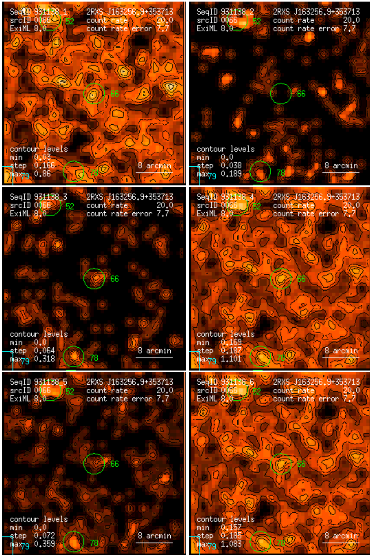
Figure 66: RASS 931138: detection 0066: band rate images, Gaussian filter: (1) PSPC channels 11 – 41, (2) 52 – 90, (3) 91 – 201, (4) 11 – 235, (5) 52 – 201, (6) 11 – 201. Broad band rates in counts/ks. Band rate contour levels in counts/ks/arcmin 2 .
