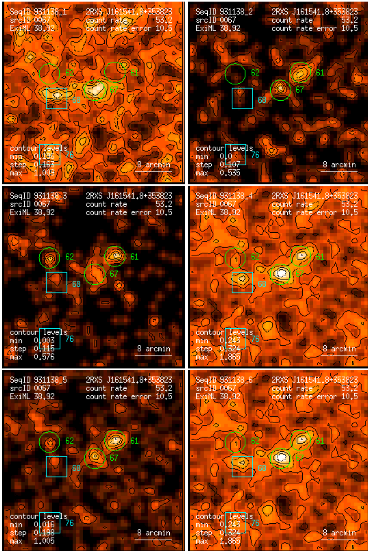
Figure 67: RASS 931138: detection 0067: band rate images, Gaussian filter: (1) PSPC channels 11 – 41, (2) 52 – 90, (3) 91 – 201, (4) 11 – 235, (5) 52 – 201, (6) 11 – 201. Broad band rates in counts/ks. Band rate contour levels in counts/ks/arcmin 2 .
