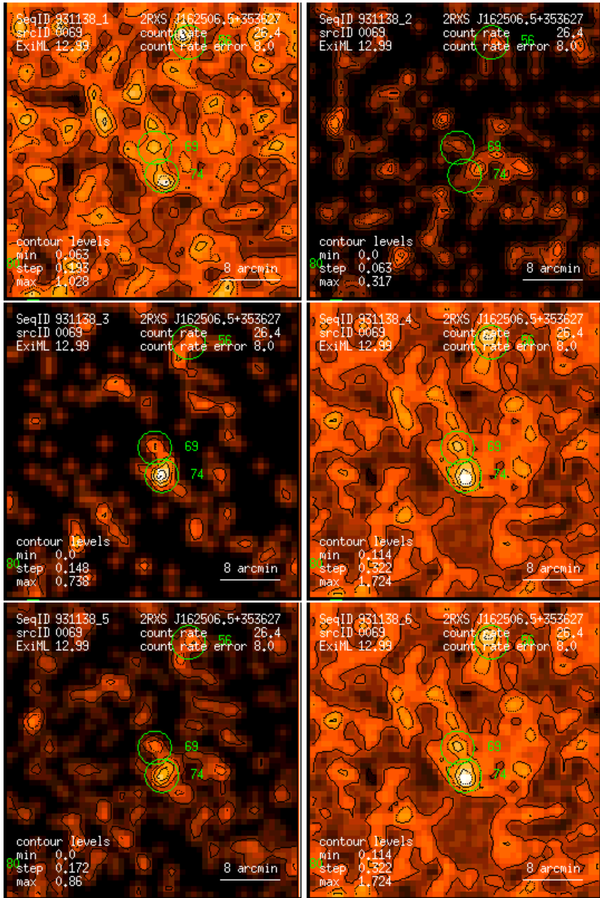
Figure 69: RASS 931138: detection 0069: band rate images, Gaussian filter: (1) PSPC channels 11 – 41, (2) 52 – 90, (3) 91 – 201, (4) 11 – 235, (5) 52 – 201, (6) 11 – 201. Broad band rates in counts/ks. Band rate contour levels in counts/ks/arcmin 2 .
