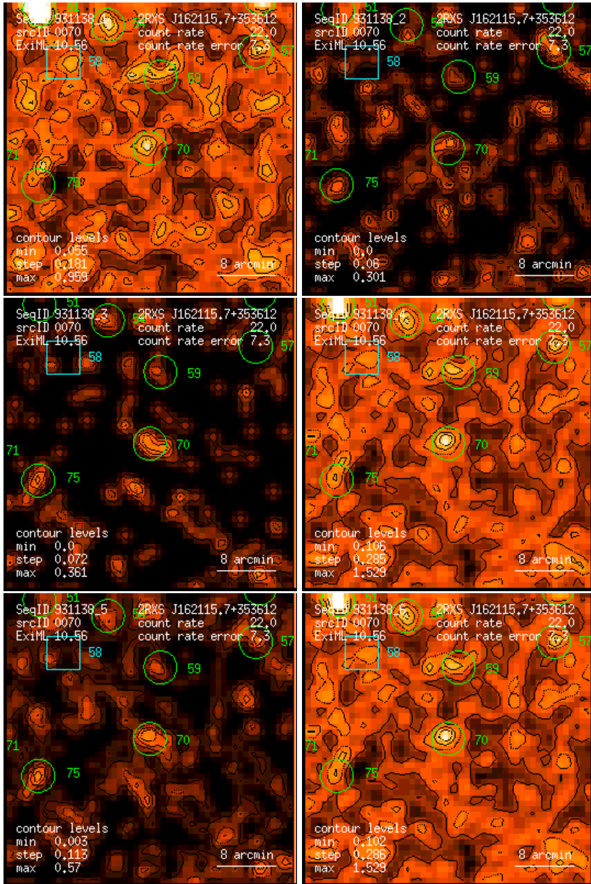
Figure 70: RASS 931138: detection 0070: band rate images, Gaussian filter: (1) PSPC channels 11 – 41, (2) 52 – 90, (3) 91 – 201, (4) 11 – 235, (5) 52 – 201, (6) 11 – 201. Broad band rates in counts/ks. Band rate contour levels in counts/ks/arcmin 2 .
