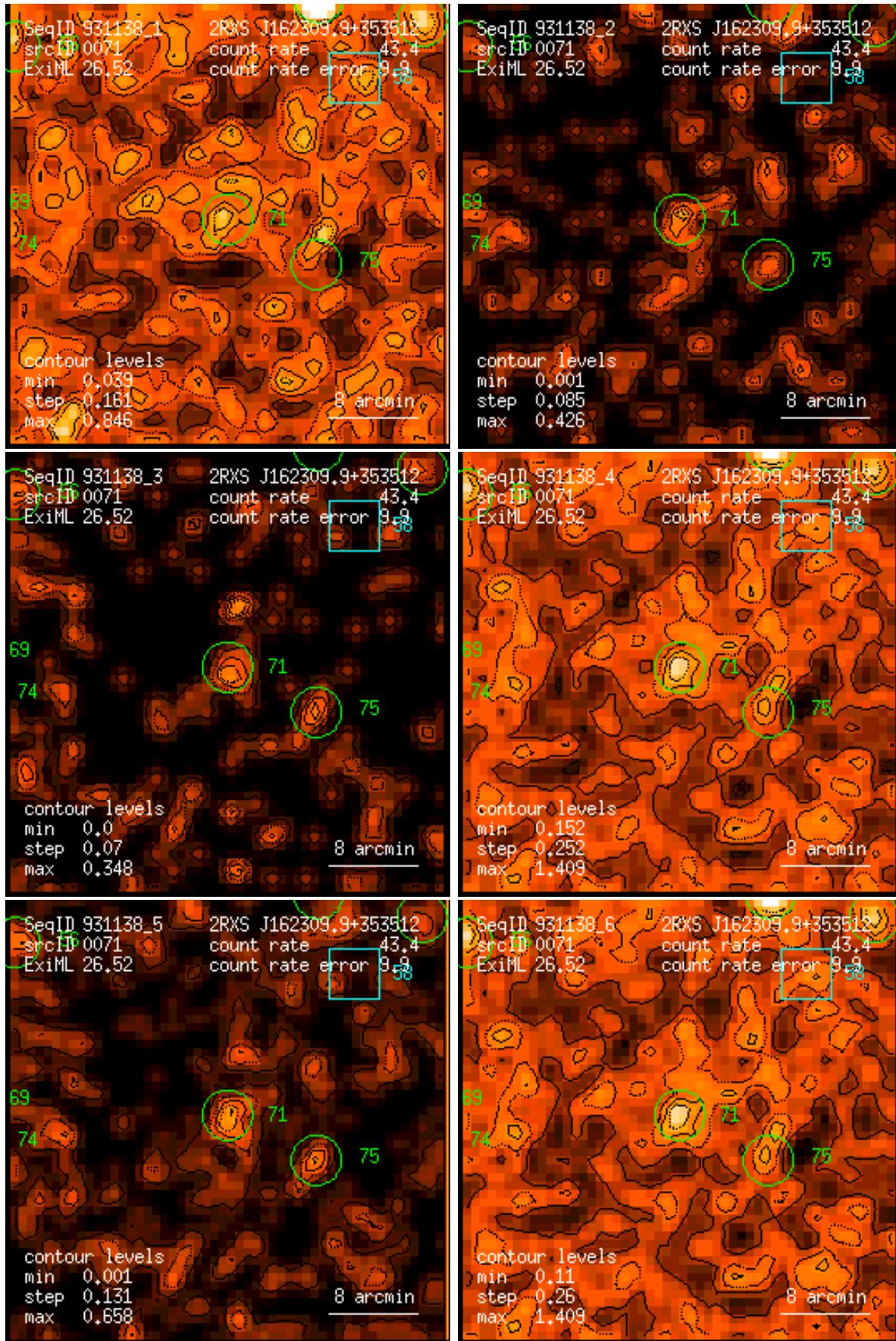
Figure 71: RASS 931138: detection 0071: band rate images, Gaussian filter: (1) PSPC channels 11 – 41, (2) 52 – 90, (3) 91 – 201, (4) 11 – 235, (5) 52 – 201, (6) 11 – 201. Broad band rates in counts/ks. Band rate contour levels in counts/ks/arcmin 2 .
