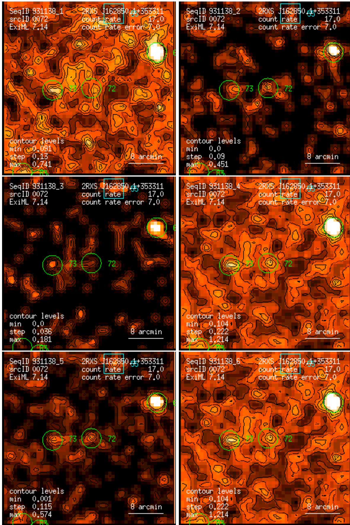
Figure 72: RASS 931138: detection 0072: band rate images, Gaussian filter: (1) PSPC channels 11 – 41, (2) 52 – 90, (3) 91 – 201, (4) 11 – 235, (5) 52 – 201, (6) 11 – 201. Broad band rates in counts/ks. Band rate contour levels in counts/ks/arcmin 2 .
