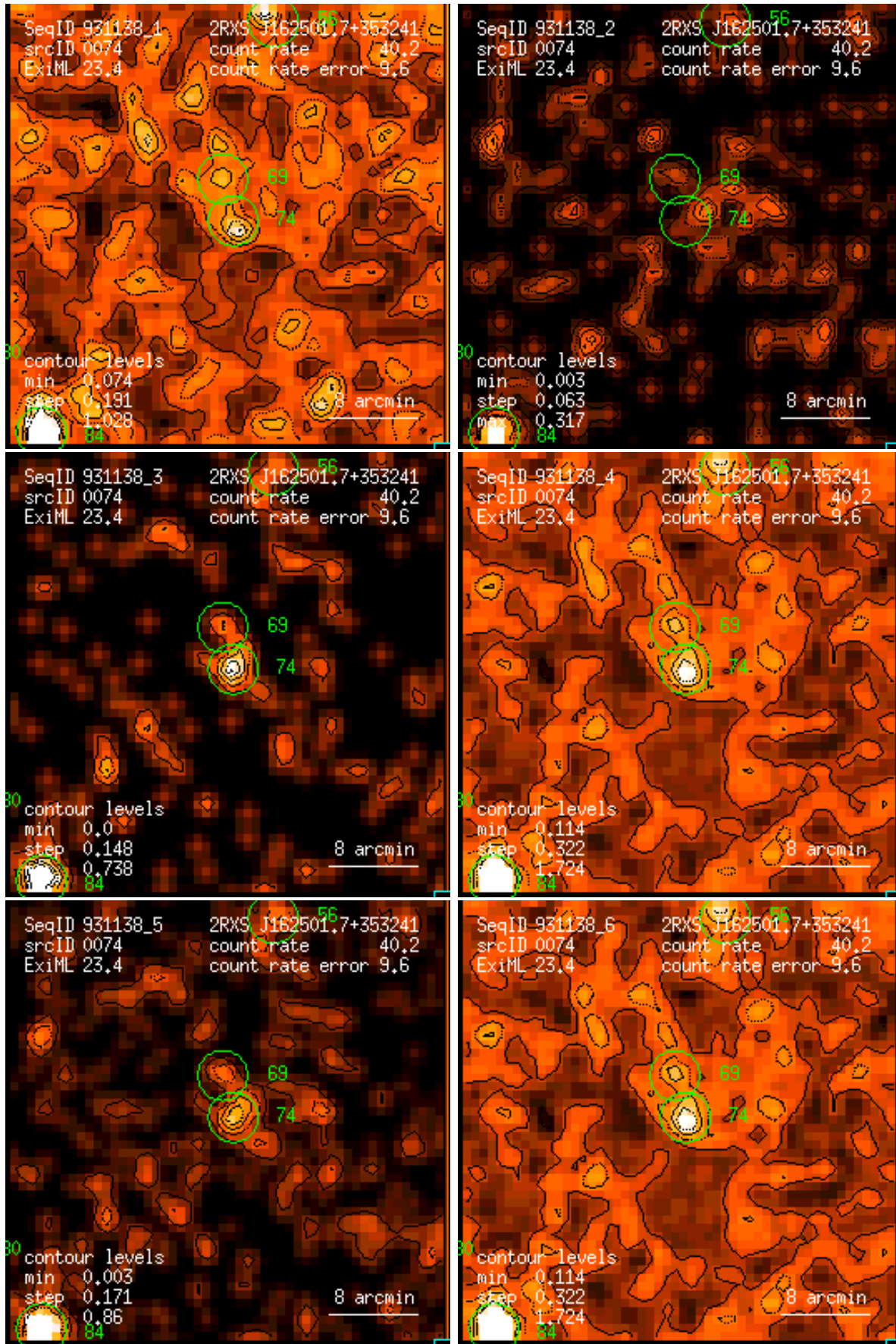
Figure 74: RASS 931138: detection 0074: band rate images, Gaussian filter: (1) PSPC channels 11 – 41, (2) 52 – 90, (3) 91 – 201, (4) 11 – 235, (5) 52 – 201, (6) 11 – 201. Broad band rates in counts/ks. Band rate contour levels in counts/ks/arcmin 2 .
