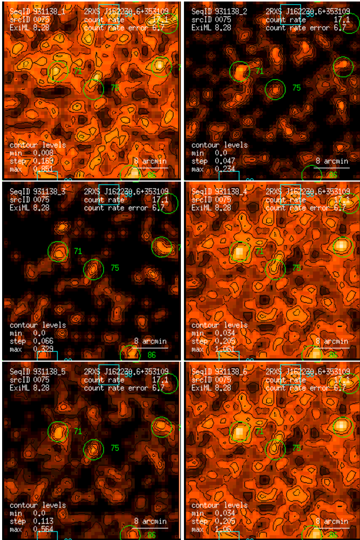
Figure 75: RASS 931138: detection 0075: band rate images, Gaussian filter: (1) PSPC channels 11 – 41, (2) 52 – 90, (3) 91 – 201, (4) 11 – 235, (5) 52 – 201, (6) 11 – 201. Broad band rates in counts/ks. Band rate contour levels in counts/ks/arcmin 2 .
