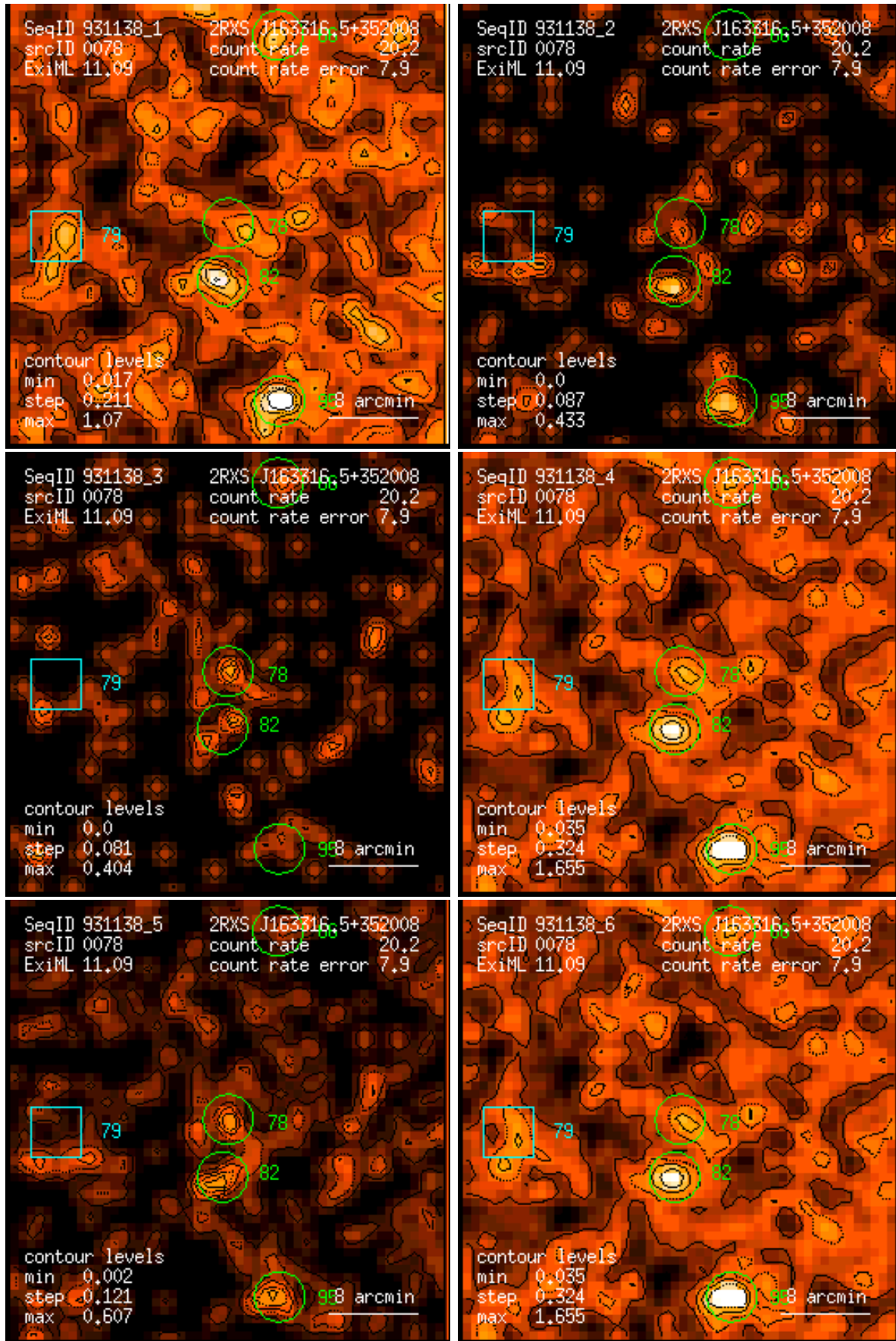
Figure 78: RASS 931138: detection 0078: band rate images, Gaussian filter: (1) PSPC channels 11 – 41, (2) 52 – 90, (3) 91 – 201, (4) 11 – 235, (5) 52 – 201, (6) 11 – 201. Broad band rates in counts/ks. Band rate contour levels in counts/ks/arcmin 2 .
