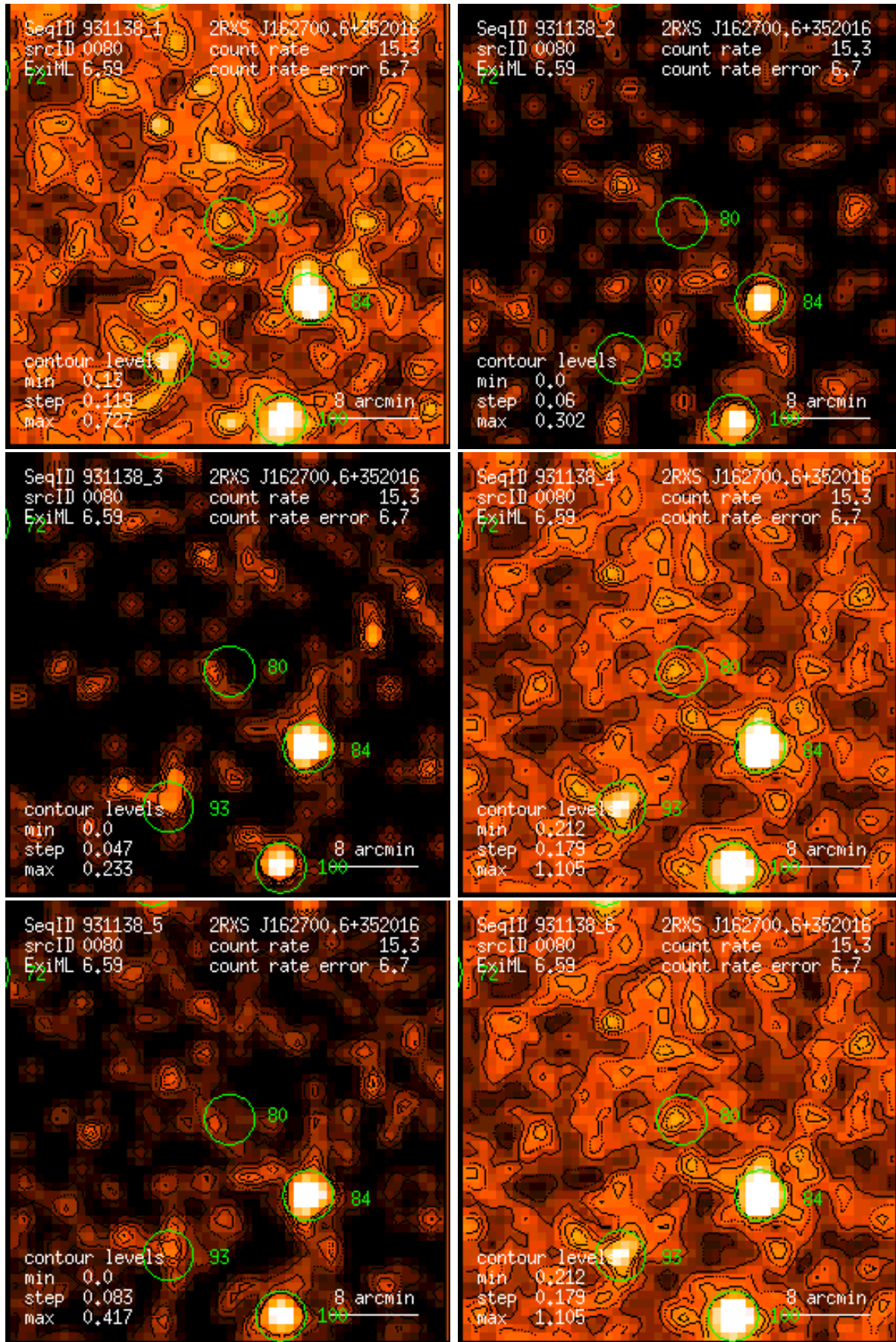
Figure 80: RASS 931138: detection 0080: band rate images, Gaussian filter: (1) PSPC channels 11 – 41, (2) 52 – 90, (3) 91 – 201, (4) 11 – 235, (5) 52 – 201, (6) 11 – 201. Broad band rates in counts/ks. Band rate contour levels in counts/ks/arcmin 2 .
