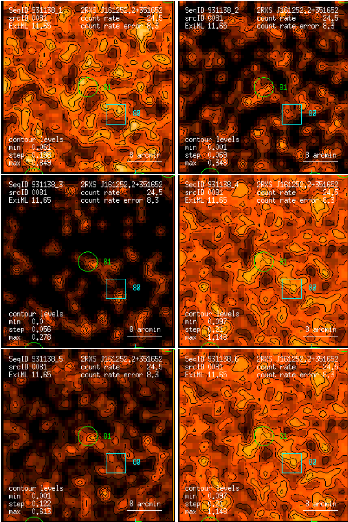
Figure 81: RASS 931138: detection 0081: band rate images, Gaussian filter: (1) PSPC channels 11 – 41, (2) 52 – 90, (3) 91 – 201, (4) 11 – 235, (5) 52 – 201, (6) 11 – 201. Broad band rates in counts/ks. Band rate contour levels in counts/ks/arcmin 2 .
