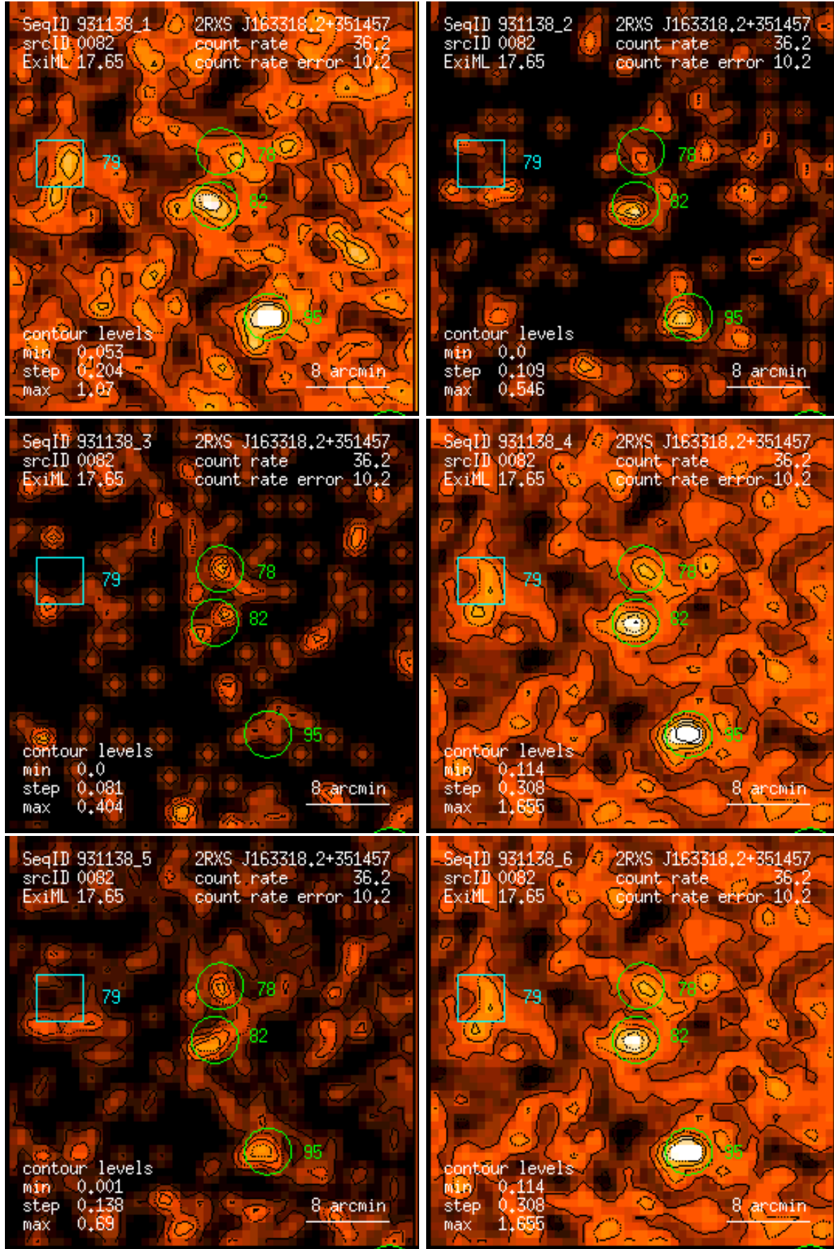
Figure 82: RASS 931138: detection 0082: band rate images, Gaussian filter: (1) PSPC channels 11 – 41, (2) 52 – 90, (3) 91 – 201, (4) 11 – 235, (5) 52 – 201, (6) 11 – 201. Broad band rates in counts/ks. Band rate contour levels in counts/ks/arcmin 2 .
