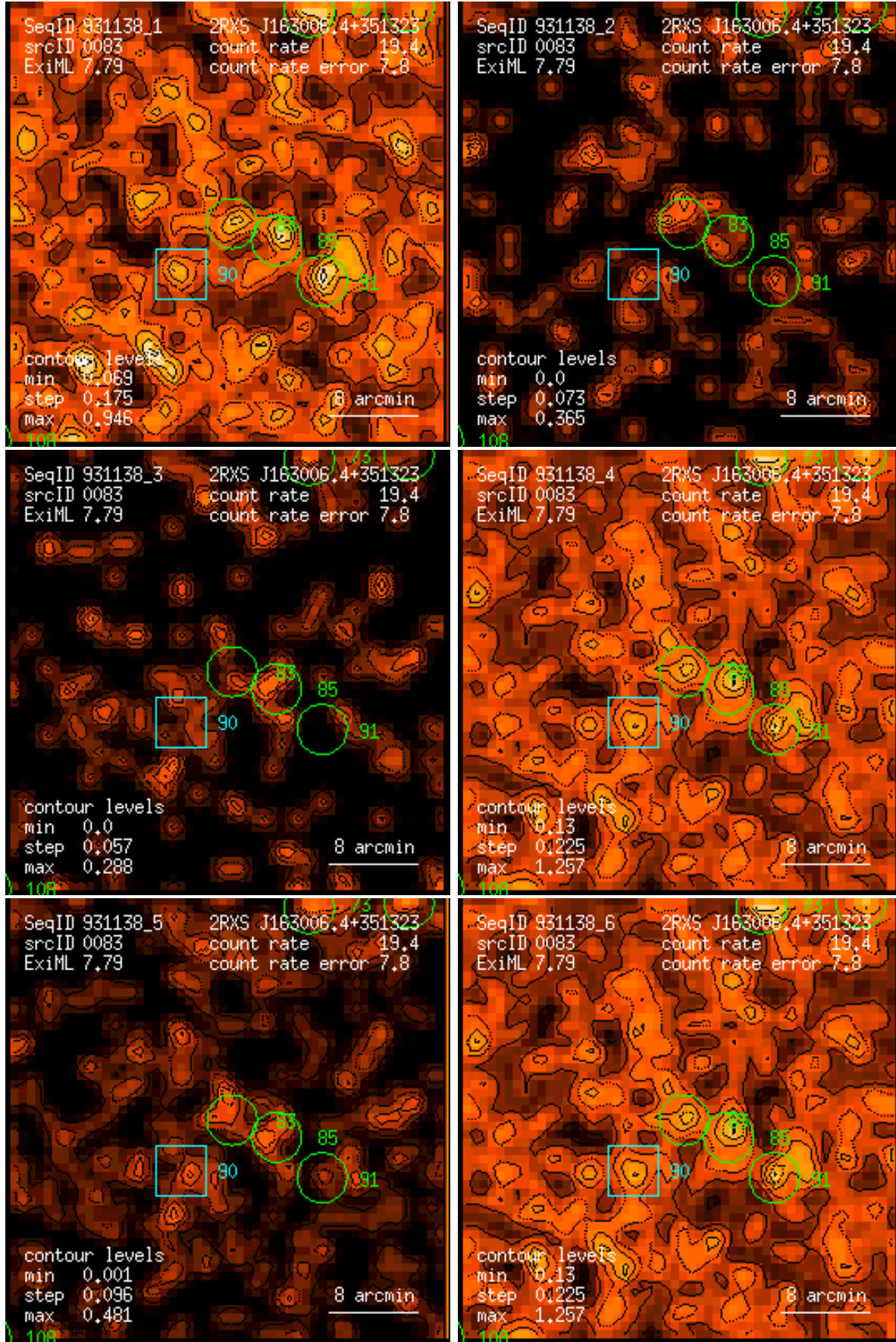
Figure 83: RASS 931138: detection 0083: band rate images, Gaussian filter: (1) PSPC channels 11 – 41, (2) 52 – 90, (3) 91 – 201, (4) 11 – 235, (5) 52 – 201, (6) 11 – 201. Broad band rates in counts/ks. Band rate contour levels in counts/ks/arcmin 2 .
