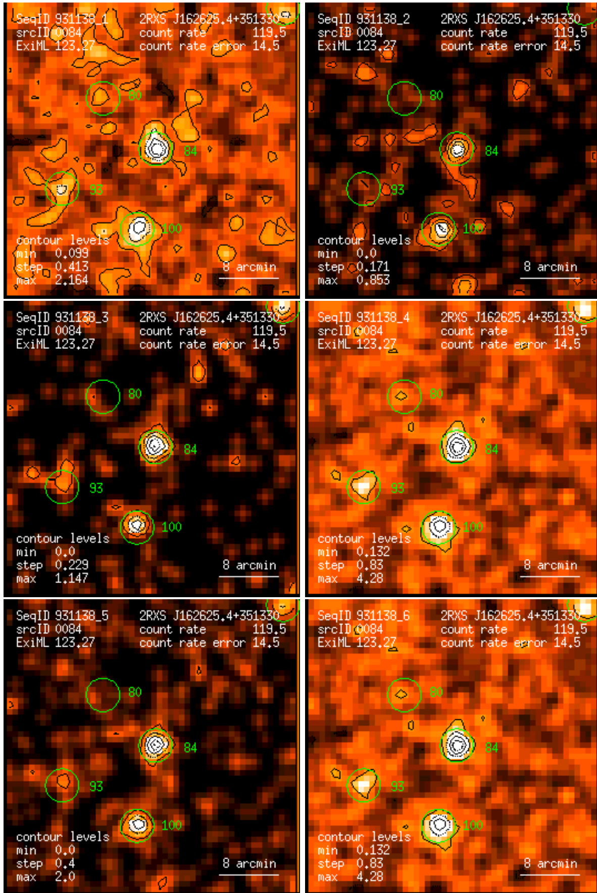
Figure 84: RASS 931138: detection 0084: band rate images, Gaussian filter: (1) PSPC channels 11 – 41, (2) 52 – 90, (3) 91 – 201, (4) 11 – 235, (5) 52 – 201, (6) 11 – 201. Broad band rates in counts/ks. Band rate contour levels in counts/ks/arcmin 2 .
