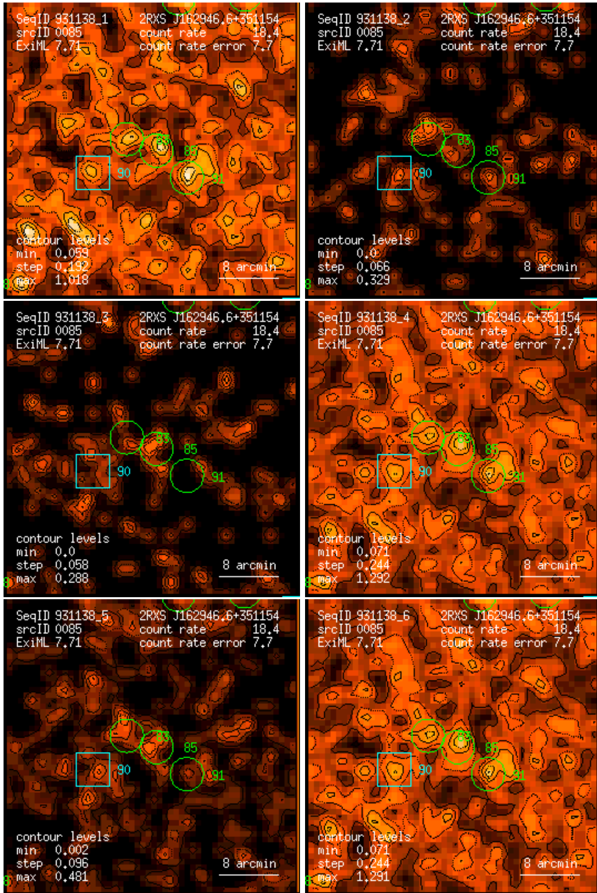
Figure 85: RASS 931138: detection 0085: band rate images, Gaussian filter: (1) PSPC channels 11 – 41, (2) 52 – 90, (3) 91 – 201, (4) 11 – 235, (5) 52 – 201, (6) 11 – 201. Broad band rates in counts/ks. Band rate contour levels in counts/ks/arcmin 2 .
