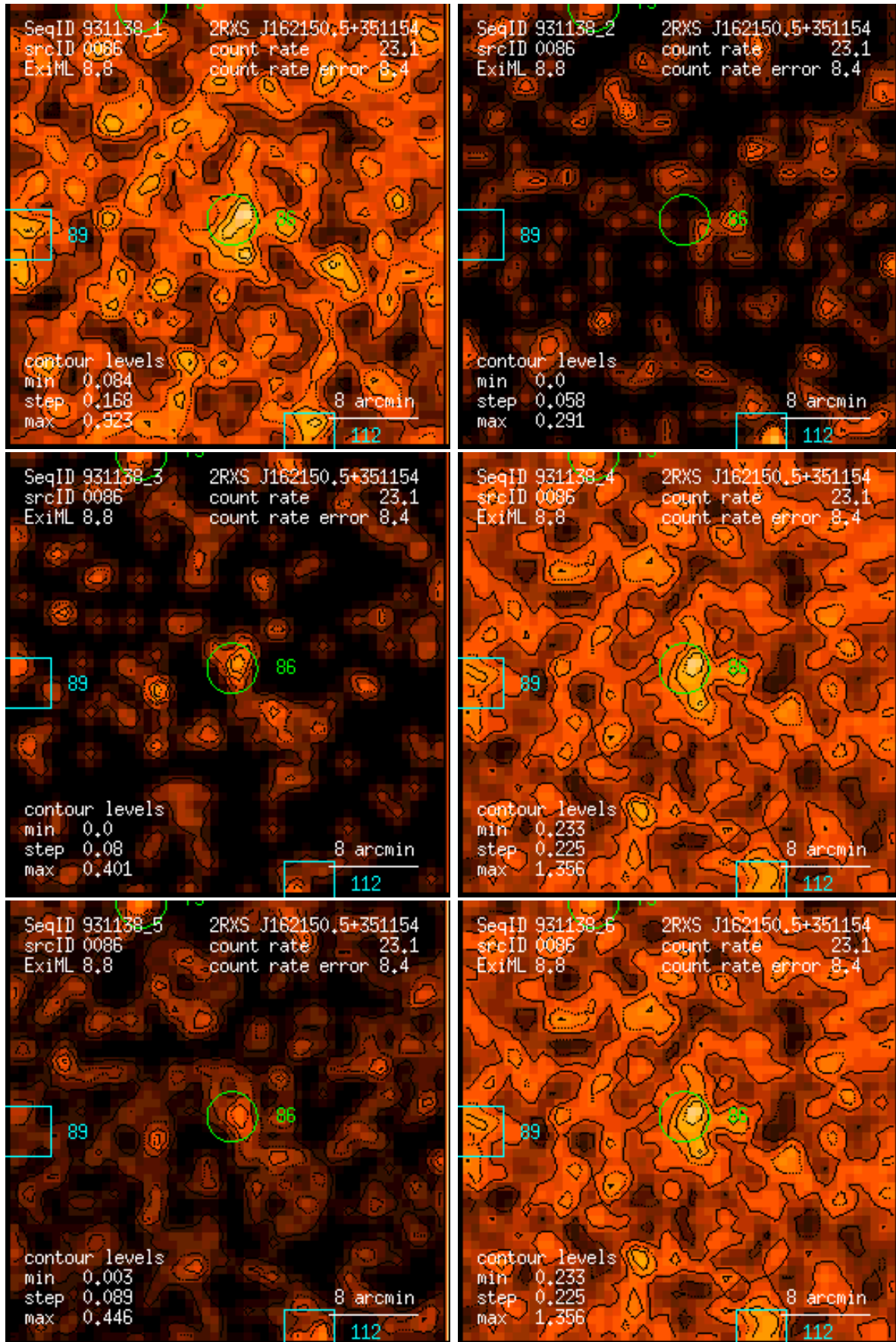
Figure 86: RASS 931138: detection 0086: band rate images, Gaussian filter: (1) PSPC channels 11 – 41, (2) 52 – 90, (3) 91 – 201, (4) 11 – 235, (5) 52 – 201, (6) 11 – 201. Broad band rates in counts/ks. Band rate contour levels in counts/ks/arcmin 2 .
