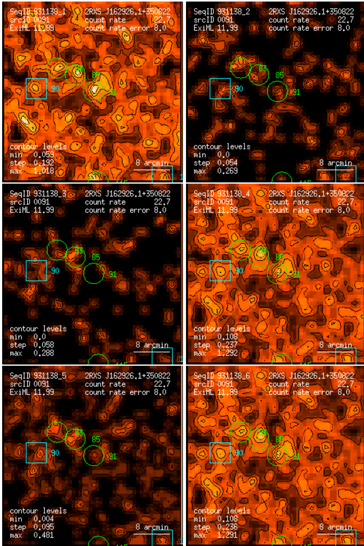
Figure 91: RASS 931138: detection 0091: band rate images, Gaussian filter: (1) PSPC channels 11 – 41, (2) 52 – 90, (3) 91 – 201, (4) 11 – 235, (5) 52 – 201, (6) 11 – 201. Broad band rates in counts/ks. Band rate contour levels in counts/ks/arcmin 2 .
