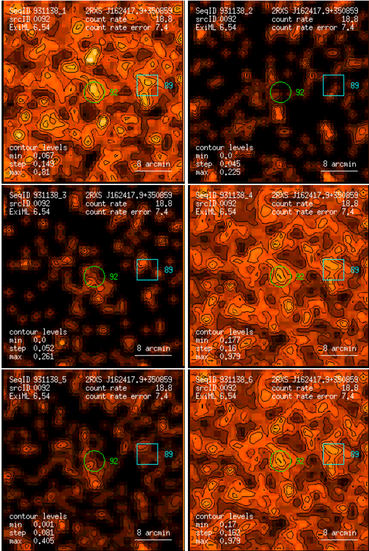
Figure 92: RASS 931138: detection 0092: band rate images, Gaussian filter: (1) PSPC channels 11 – 41, (2) 52 – 90, (3) 91 – 201, (4) 11 – 235, (5) 52 – 201, (6) 11 – 201. Broad band rates in counts/ks. Band rate contour levels in counts/ks/arcmin 2 .
