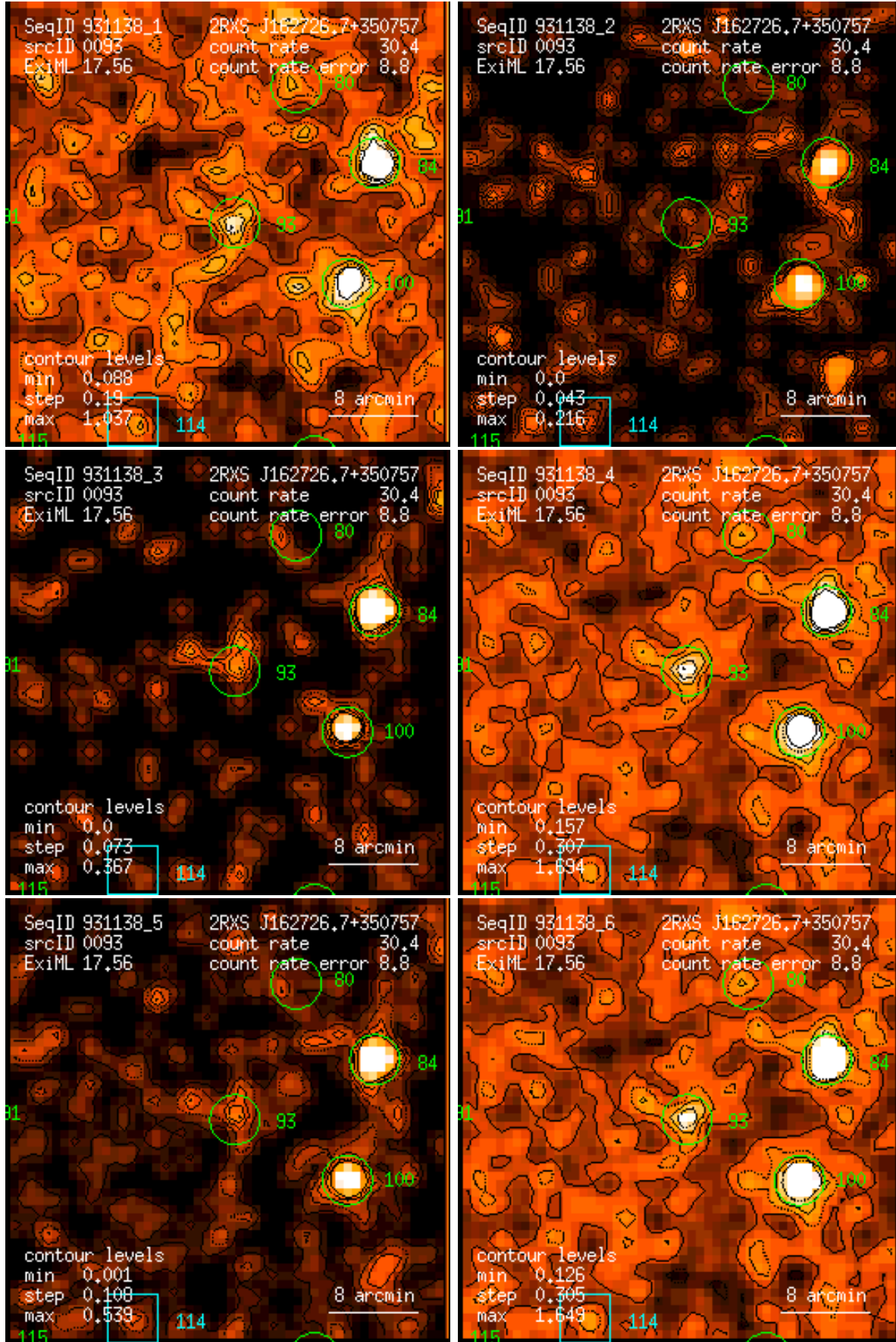
Figure 93: RASS 931138: detection 0093: band rate images, Gaussian filter: (1) PSPC channels 11 – 41, (2) 52 – 90, (3) 91 – 201, (4) 11 – 235, (5) 52 – 201, (6) 11 – 201. Broad band rates in counts/ks. Band rate contour levels in counts/ks/arcmin 2 .
