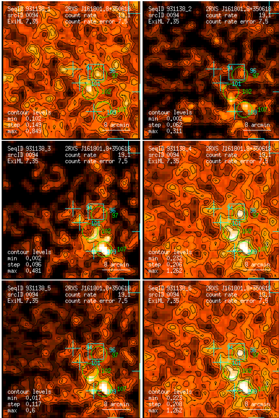
Figure 94: RASS 931138: detection 0094: band rate images, Gaussian filter: (1) PSPC channels 11 – 41, (2) 52 – 90, (3) 91 – 201, (4) 11 – 235, (5) 52 – 201, (6) 11 – 201. Broad band rates in counts/ks. Band rate contour levels in counts/ks/arcmin 2 .
