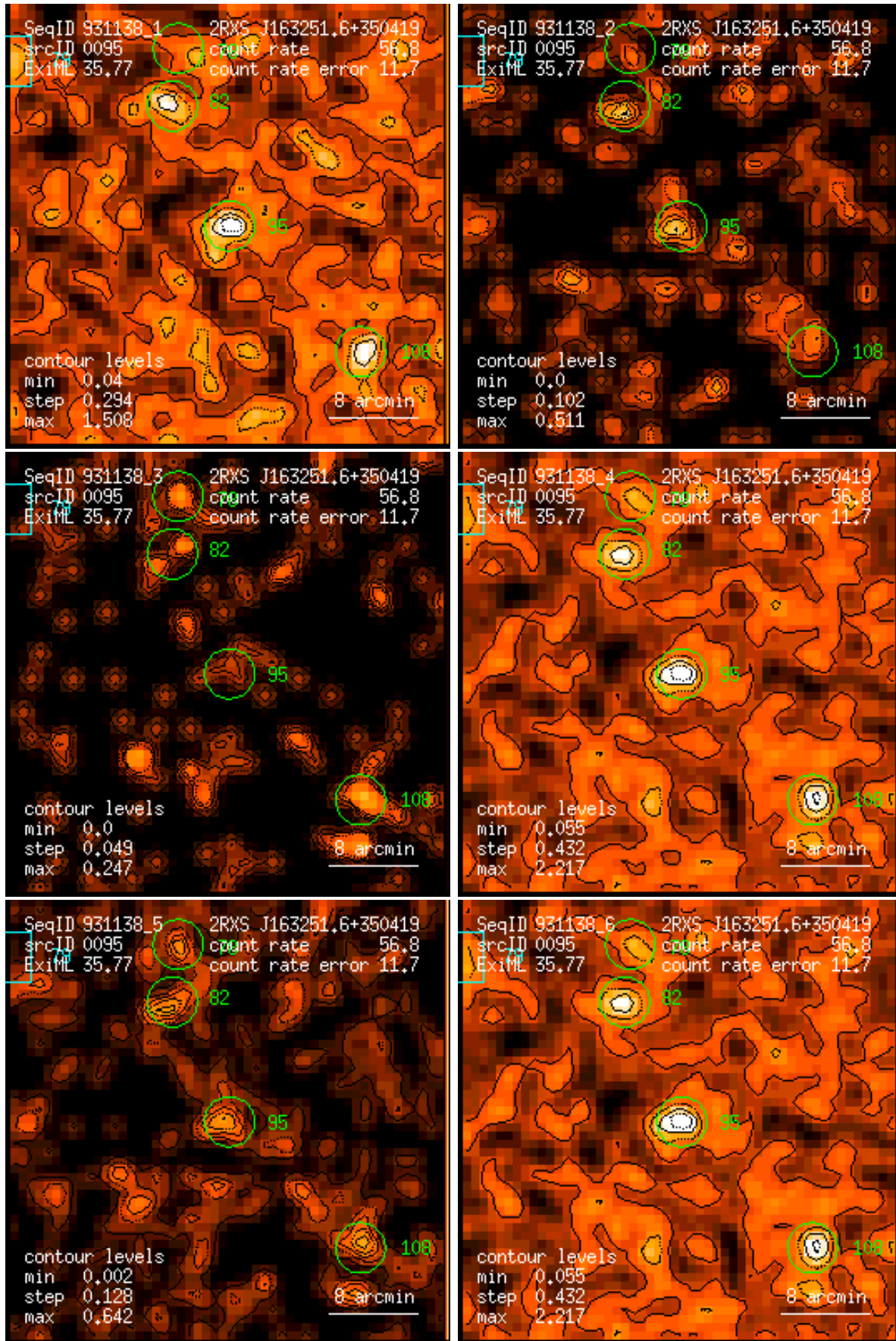
Figure 95: RASS 931138: detection 0095: band rate images, Gaussian filter: (1) PSPC channels 11 – 41, (2) 52 – 90, (3) 91 – 201, (4) 11 – 235, (5) 52 – 201, (6) 11 – 201. Broad band rates in counts/ks. Band rate contour levels in counts/ks/arcmin 2 .
