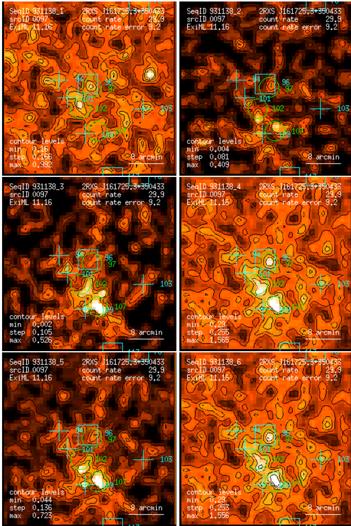
Figure 97: RASS 931138: detection 0097: band rate images, Gaussian filter: (1) PSPC channels 11 – 41, (2) 52 – 90, (3) 91 – 201, (4) 11 – 235, (5) 52 – 201, (6) 11 – 201. Broad band rates in counts/ks. Band rate contour levels in counts/ks/arcmin 2 .
