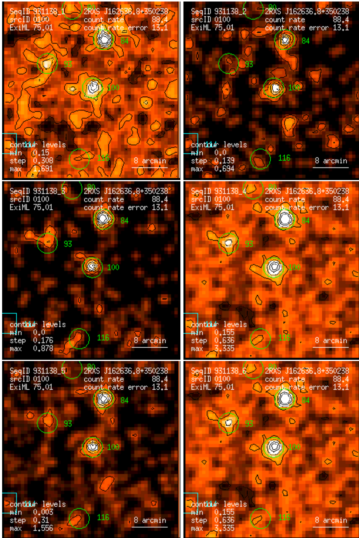
Figure 100: RASS 931138: detection 0100: band rate images, Gaussian filter: (1) PSPC channels 11 – 41, (2) 52 – 90, (3) 91 – 201, (4) 11 – 235, (5) 52 – 201, (6) 11 – 201. Broad band rates in counts/ks. Band rate contour levels in counts/ks/arcmin 2 .
