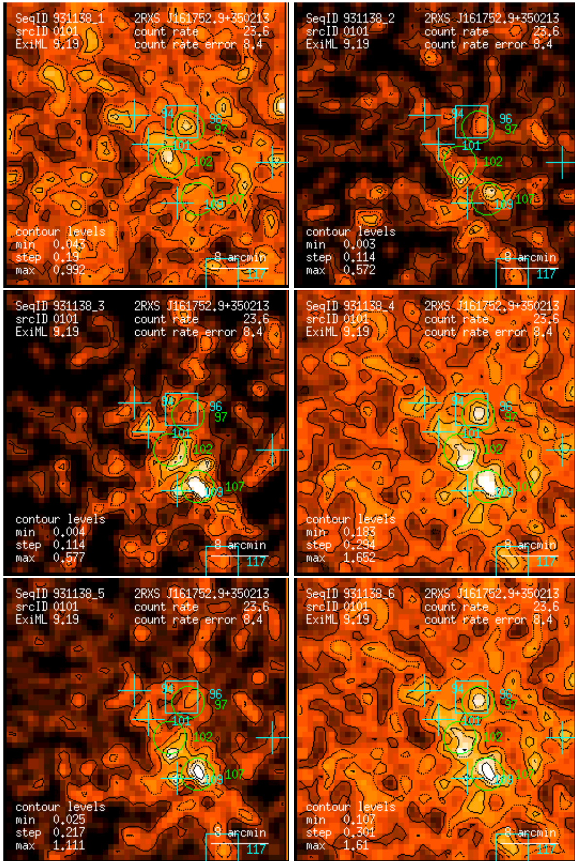
Figure 101: RASS 931138: detection 0101: band rate images, Gaussian filter: (1) PSPC channels 11 – 41, (2) 52 – 90, (3) 91 – 201, (4) 11 – 235, (5) 52 – 201, (6) 11 – 201. Broad band rates in counts/ks. Band rate contour levels in counts/ks/arcmin 2 .
