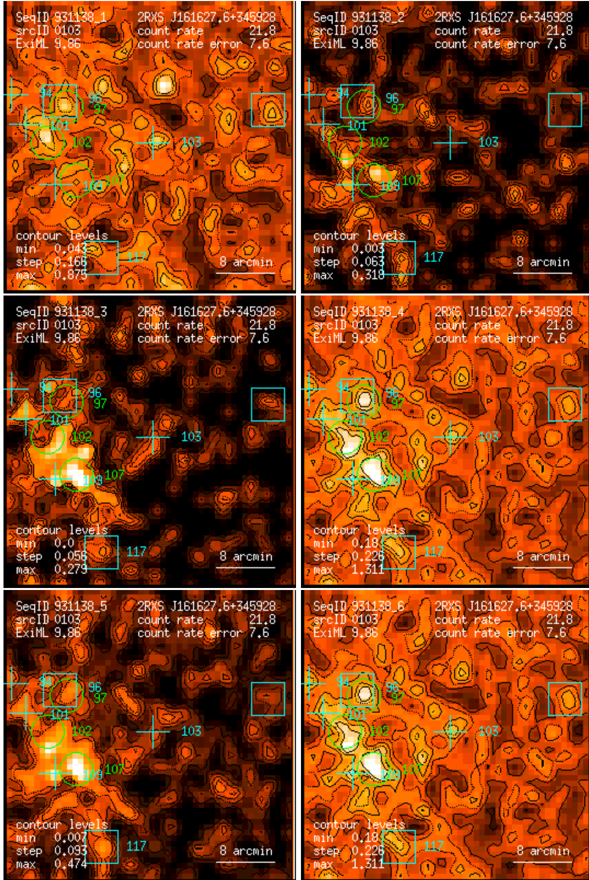
Figure 103: RASS 931138: detection 0103: band rate images, Gaussian filter: (1) PSPC channels 11 – 41, (2) 52 – 90, (3) 91 – 201, (4) 11 – 235, (5) 52 – 201, (6) 11 – 201. Broad band rates in counts/ks. Band rate contour levels in counts/ks/arcmin 2 .
