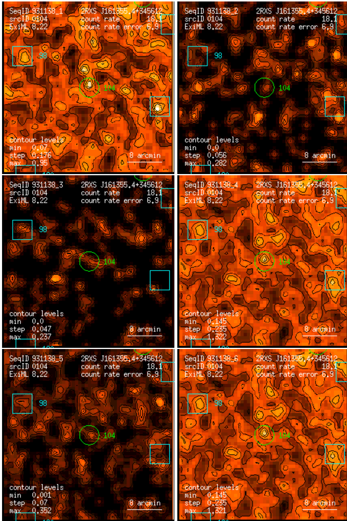
Figure 104: RASS 931138: detection 0104: band rate images, Gaussian filter: (1) PSPC channels 11 – 41, (2) 52 – 90, (3) 91 – 201, (4) 11 – 235, (5) 52 – 201, (6) 11 – 201. Broad band rates in counts/ks. Band rate contour levels in counts/ks/arcmin 2 .
