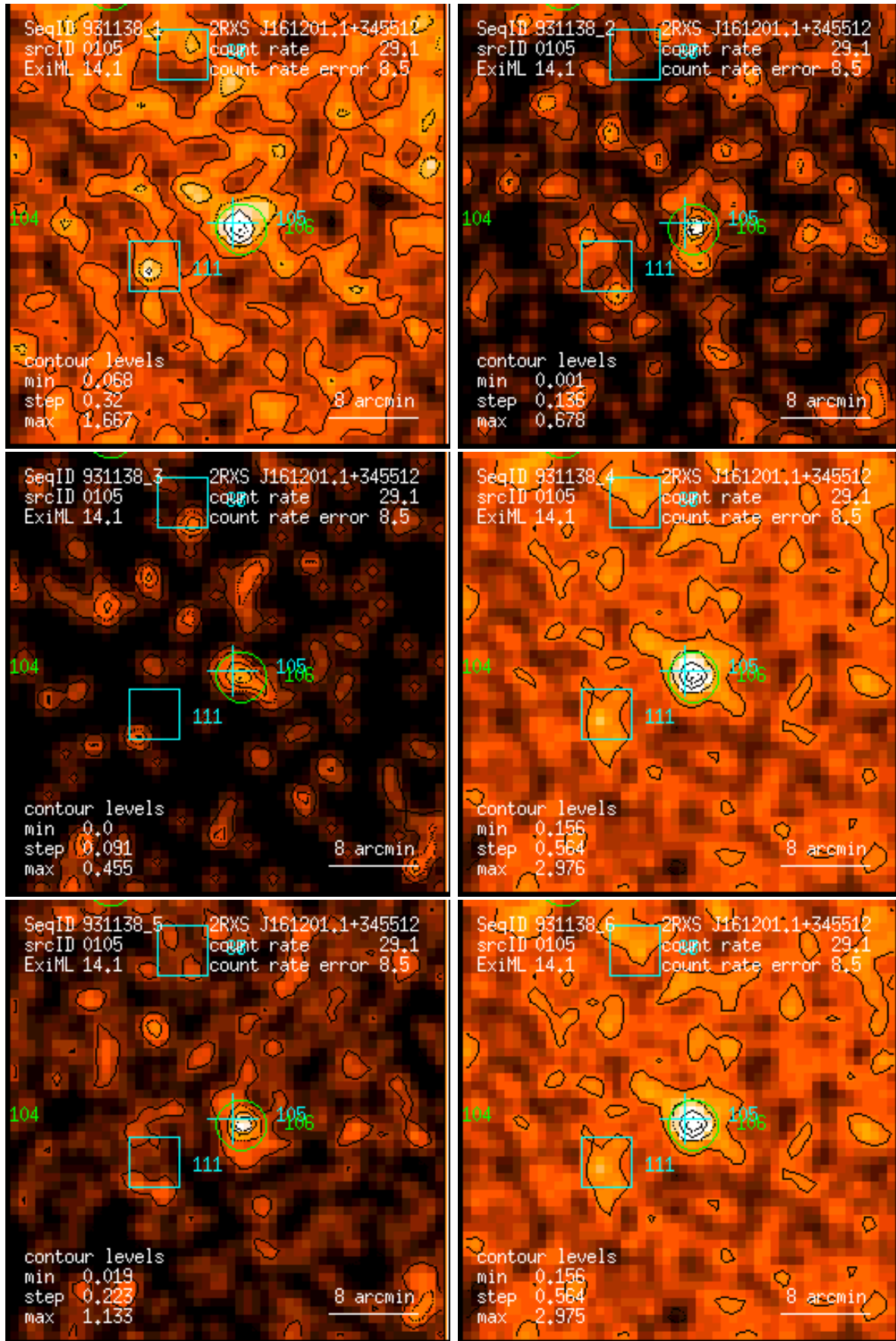
Figure 105: RASS 931138: detection 0105: band rate images, Gaussian filter: (1) PSPC channels 11 – 41, (2) 52 – 90, (3) 91 – 201, (4) 11 – 235, (5) 52 – 201, (6) 11 – 201. Broad band rates in counts/ks. Band rate contour levels in counts/ks/arcmin 2 .
