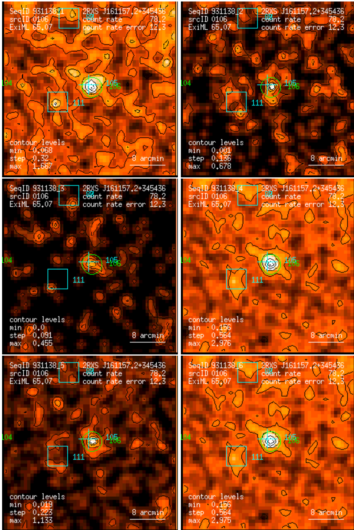
Figure 106: RASS 931138: detection 0106: band rate images, Gaussian filter: (1) PSPC channels 11 – 41, (2) 52 – 90, (3) 91 – 201, (4) 11 – 235, (5) 52 – 201, (6) 11 – 201. Broad band rates in counts/ks. Band rate contour levels in counts/ks/arcmin 2 .
