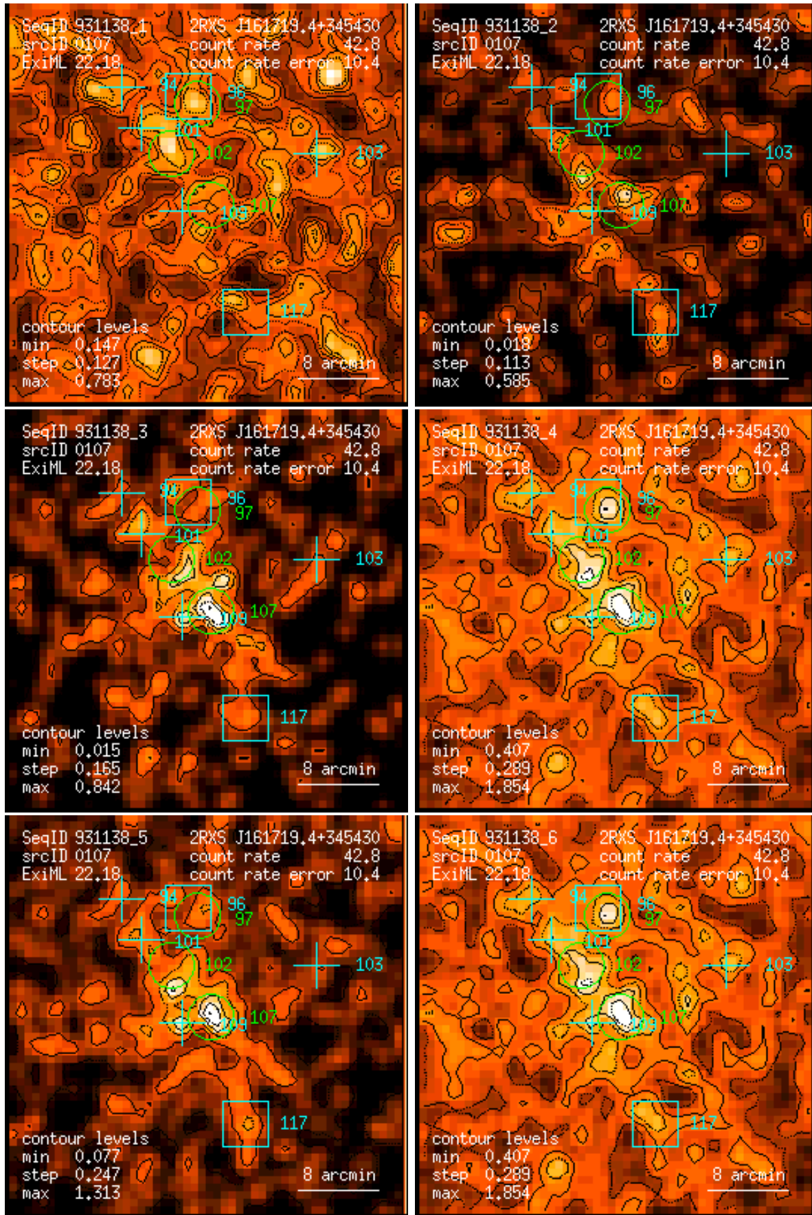
Figure 107: RASS 931138: detection 0107: band rate images, Gaussian filter: (1) PSPC channels 11 – 41, (2) 52 – 90, (3) 91 – 201, (4) 11 – 235, (5) 52 – 201, (6) 11 – 201. Broad band rates in counts/ks. Band rate contour levels in counts/ks/arcmin 2 .
