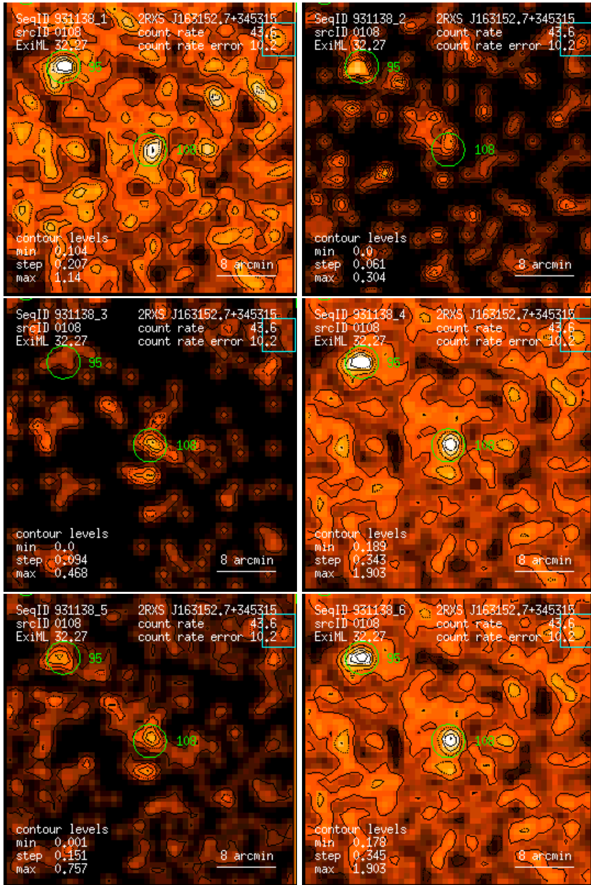
Figure 108: RASS 931138: detection 0108: band rate images, Gaussian filter: (1) PSPC channels 11 – 41, (2) 52 – 90, (3) 91 – 201, (4) 11 – 235, (5) 52 – 201, (6) 11 – 201. Broad band rates in counts/ks. Band rate contour levels in counts/ks/arcmin 2 .
