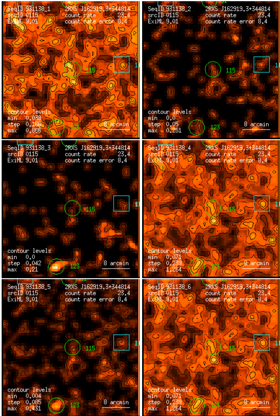
Figure 115: RASS 931138: detection 0115: band rate images, Gaussian filter: (1) PSPC channels 11 – 41, (2) 52 – 90, (3) 91 – 201, (4) 11 – 235, (5) 52 – 201, (6) 11 – 201. Broad band rates in counts/ks. Band rate contour levels in counts/ks/arcmin 2 .
