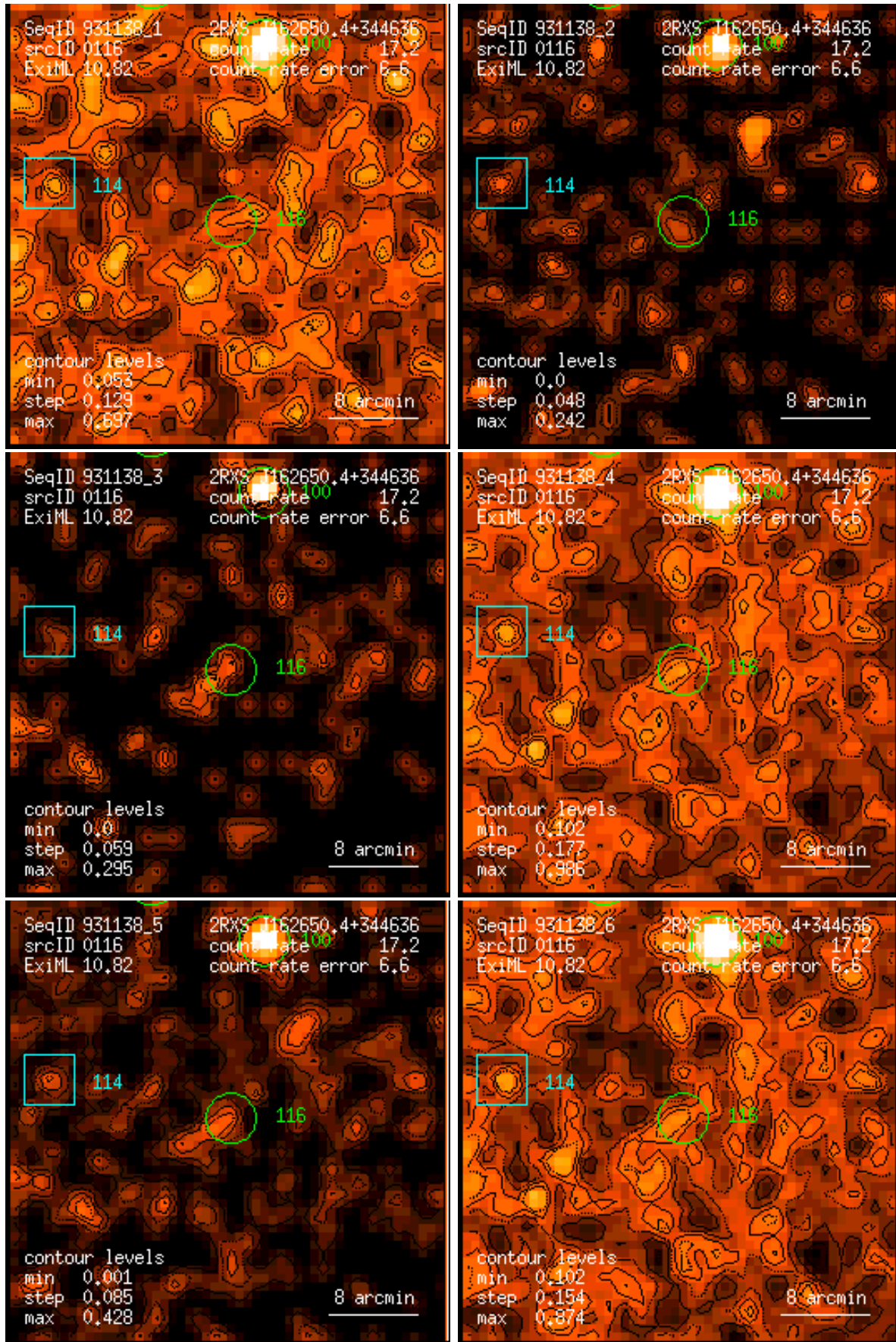
Figure 116: RASS 931138: detection 0116: band rate images, Gaussian filter: (1) PSPC channels 11 – 41, (2) 52 – 90, (3) 91 – 201, (4) 11 – 235, (5) 52 – 201, (6) 11 – 201. Broad band rates in counts/ks. Band rate contour levels in counts/ks/arcmin 2 .
