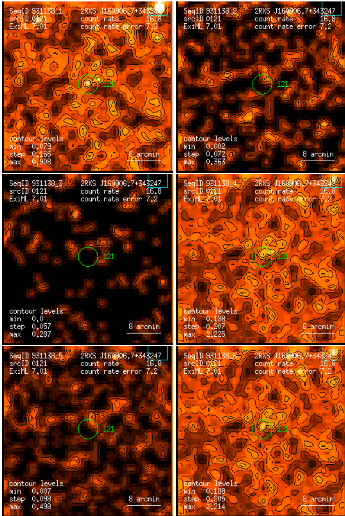
Figure 121: RASS 931138: detection 0121: band rate images, Gaussian filter: (1) PSPC channels 11 – 41, (2) 52 – 90, (3) 91 – 201, (4) 11 – 235, (5) 52 – 201, (6) 11 – 201. Broad band rates in counts/ks. Band rate contour levels in counts/ks/arcmin 2 .
