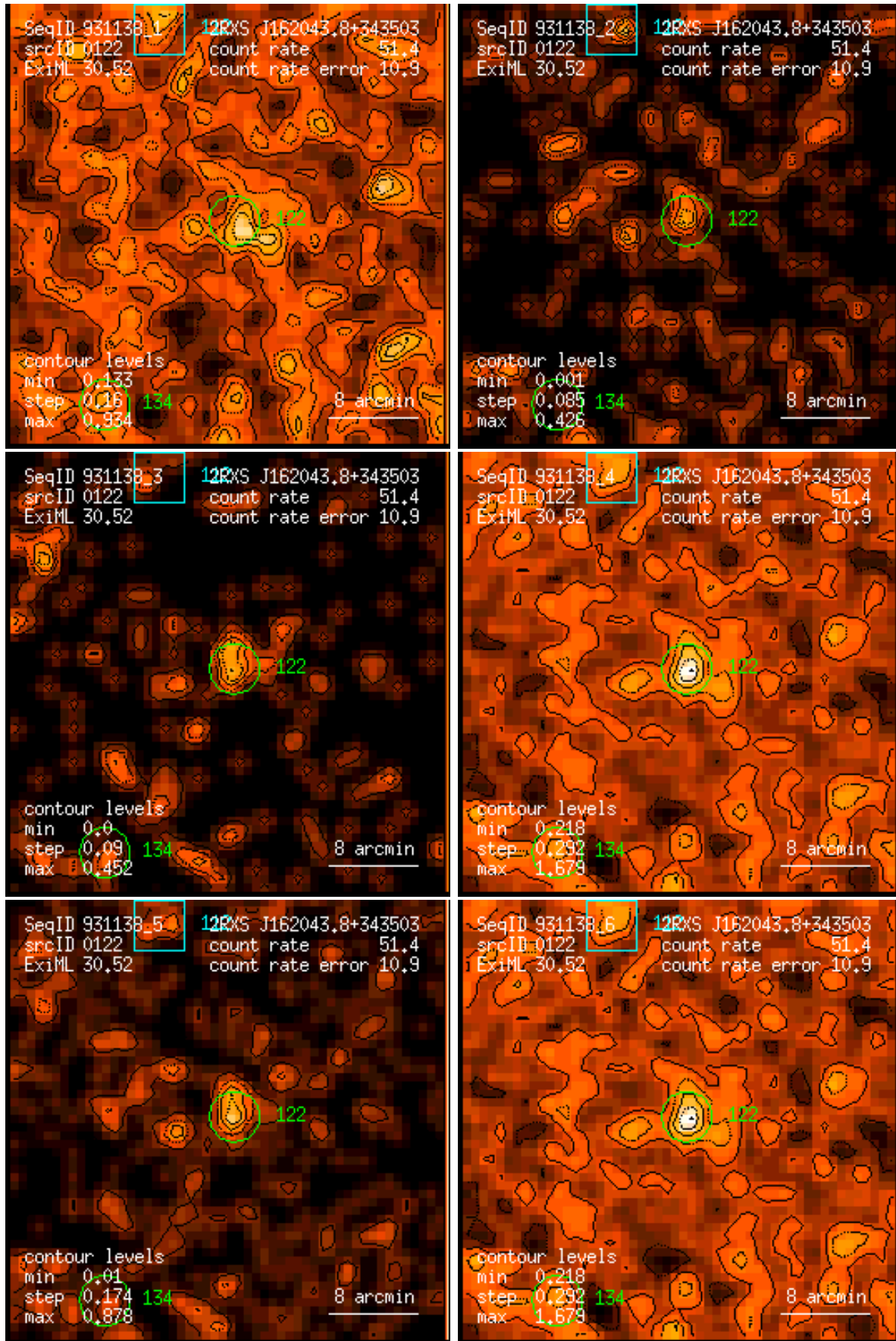
Figure 122: RASS 931138: detection 0122: band rate images, Gaussian filter: (1) PSPC channels 11 – 41, (2) 52 – 90, (3) 91 – 201, (4) 11 – 235, (5) 52 – 201, (6) 11 – 201. Broad band rates in counts/ks. Band rate contour levels in counts/ks/arcmin 2 .
