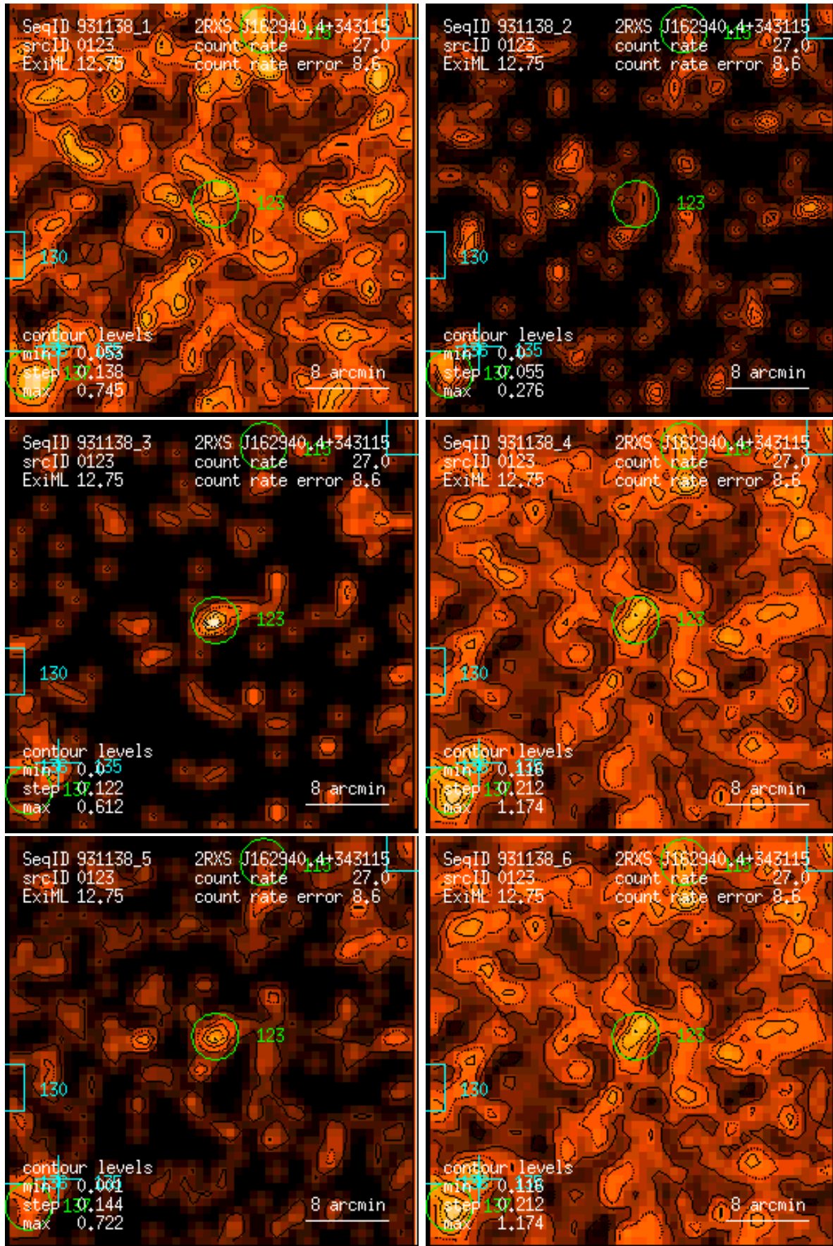
Figure 123: RASS 931138: detection 0123: band rate images, Gaussian filter: (1) PSPC channels 11 – 41, (2) 52 – 90, (3) 91 – 201, (4) 11 – 235, (5) 52 – 201, (6) 11 – 201. Broad band rates in counts/ks. Band rate contour levels in counts/ks/arcmin 2 .
