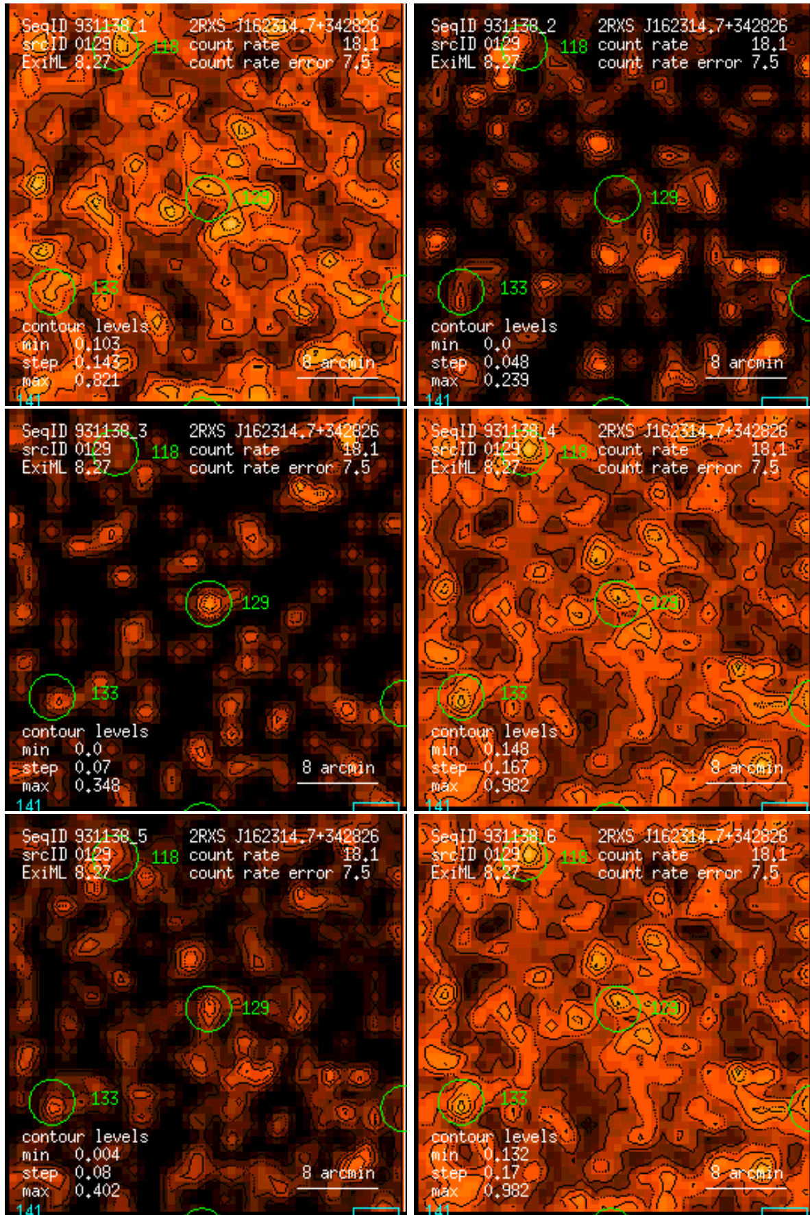
Figure 129: RASS 931138: detection 0129: band rate images, Gaussian filter: (1) PSPC channels 11 – 41, (2) 52 – 90, (3) 91 – 201, (4) 11 – 235, (5) 52 – 201, (6) 11 – 201. Broad band rates in counts/ks. Band rate contour levels in counts/ks/arcmin 2 .
