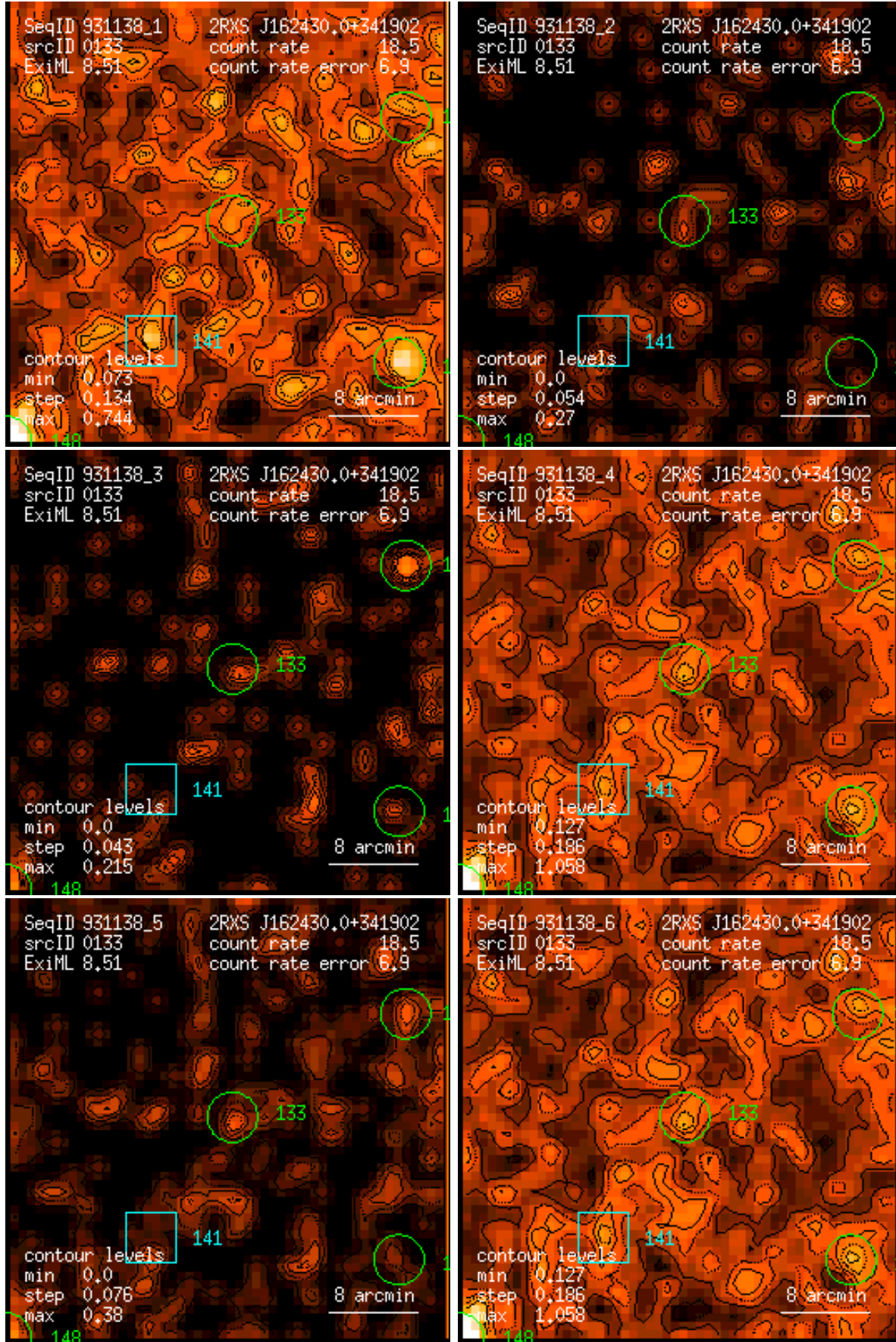
Figure 133: RASS 931138: detection 0133: band rate images, Gaussian filter: (1) PSPC channels 11 – 41, (2) 52 – 90, (3) 91 – 201, (4) 11 – 235, (5) 52 – 201, (6) 11 – 201. Broad band rates in counts/ks. Band rate contour levels in counts/ks/arcmin 2 .
