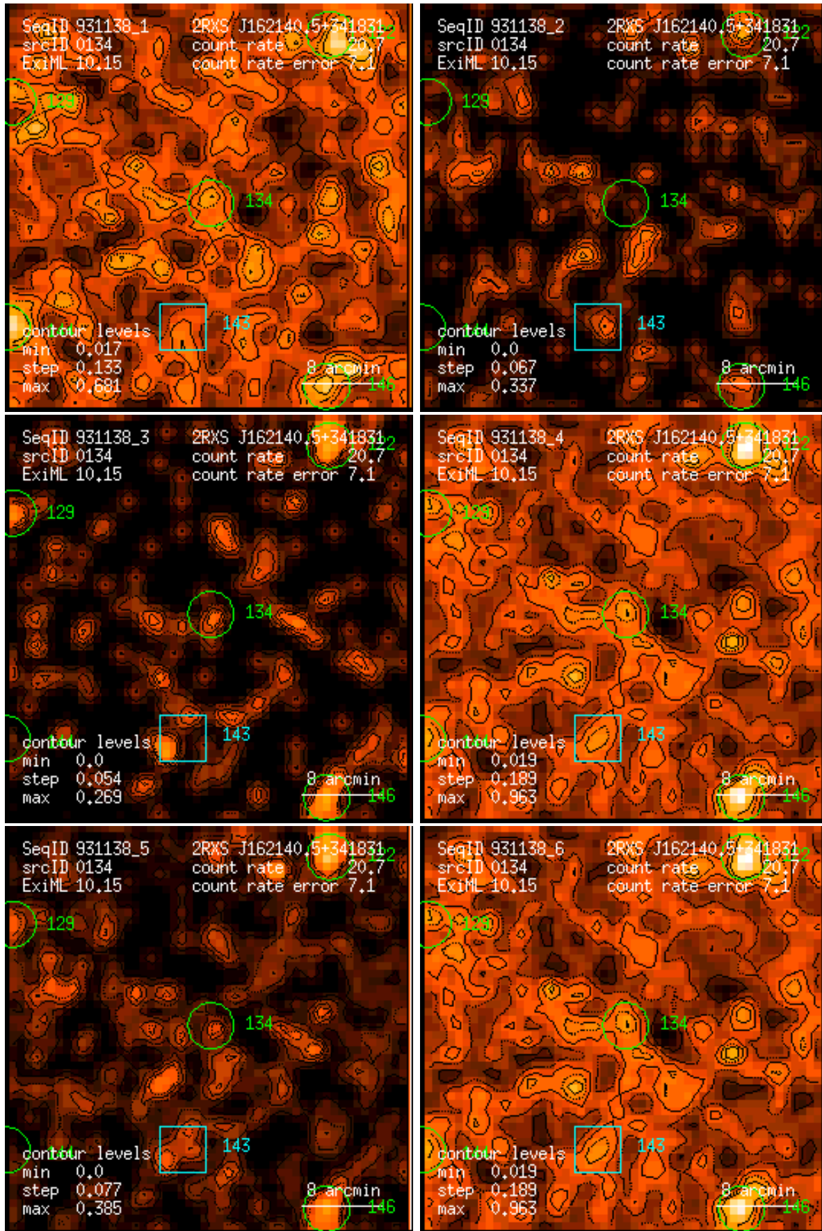
Figure 134: RASS 931138: detection 0134: band rate images, Gaussian filter: (1) PSPC channels 11 – 41, (2) 52 – 90, (3) 91 – 201, (4) 11 – 235, (5) 52 – 201, (6) 11 – 201. Broad band rates in counts/ks. Band rate contour levels in counts/ks/arcmin 2 .
