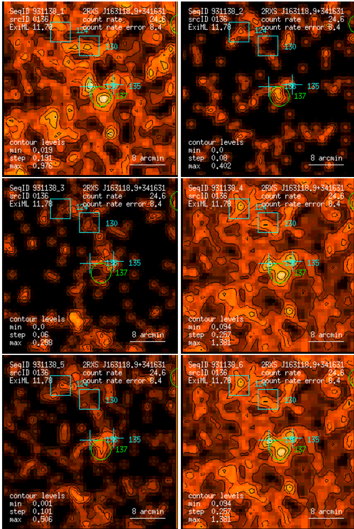
Figure 136: RASS 931138: detection 0136: band rate images, Gaussian filter: (1) PSPC channels 11 – 41, (2) 52 – 90, (3) 91 – 201, (4) 11 – 235, (5) 52 – 201, (6) 11 – 201. Broad band rates in counts/ks. Band rate contour levels in counts/ks/arcmin 2 .
