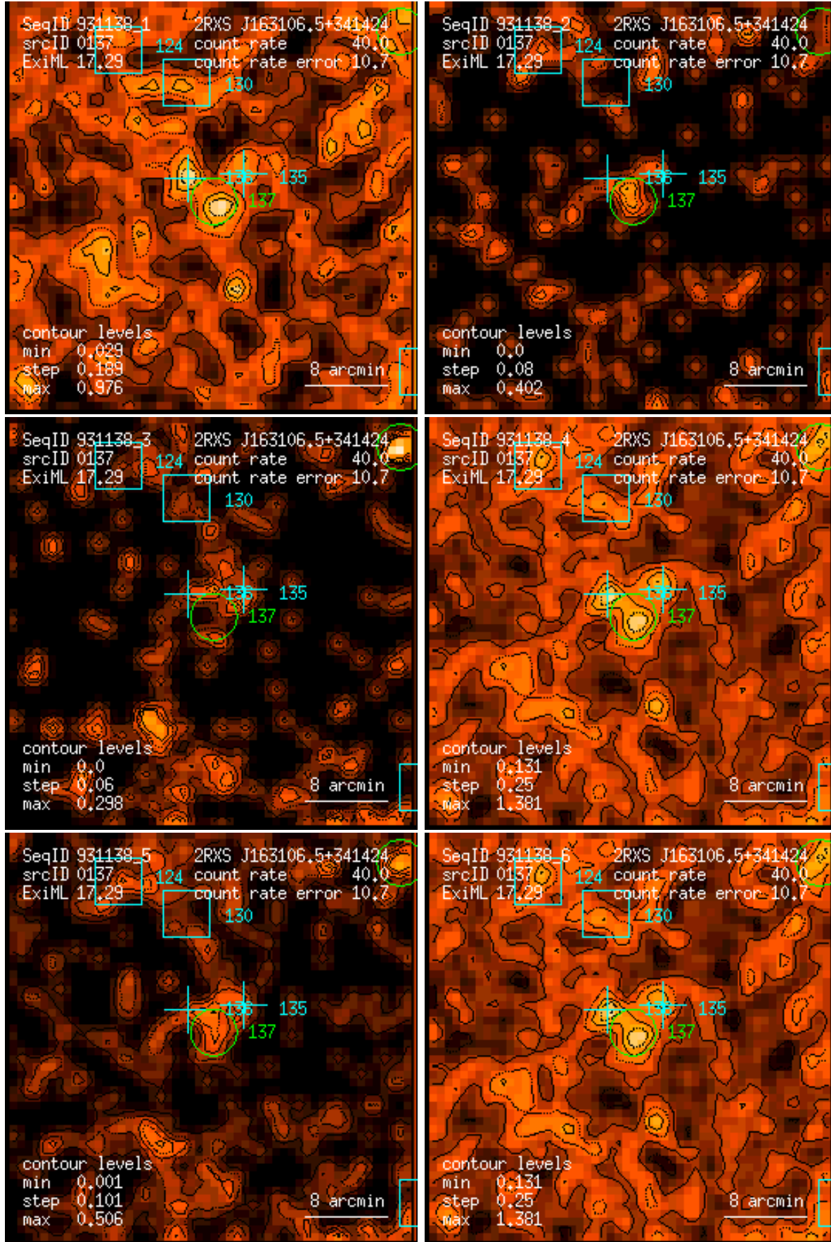
Figure 137: RASS 931138: detection 0137: band rate images, Gaussian filter: (1) PSPC channels 11 – 41, (2) 52 – 90, (3) 91 – 201, (4) 11 – 235, (5) 52 – 201, (6) 11 – 201. Broad band rates in counts/ks. Band rate contour levels in counts/ks/arcmin 2 .
