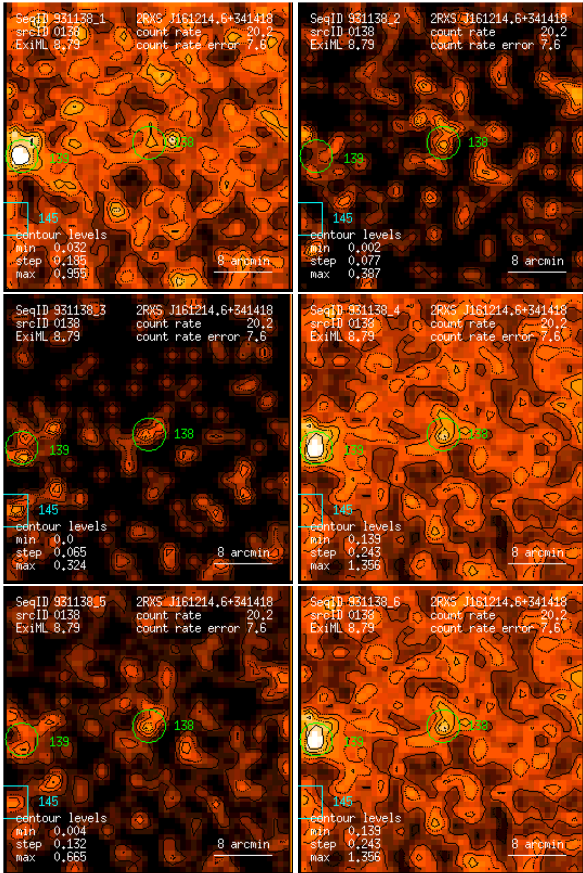
Figure 138: RASS 931138: detection 0138: band rate images, Gaussian filter: (1) PSPC channels 11 – 41, (2) 52 – 90, (3) 91 – 201, (4) 11 – 235, (5) 52 – 201, (6) 11 – 201. Broad band rates in counts/ks. Band rate contour levels in counts/ks/arcmin 2 .
