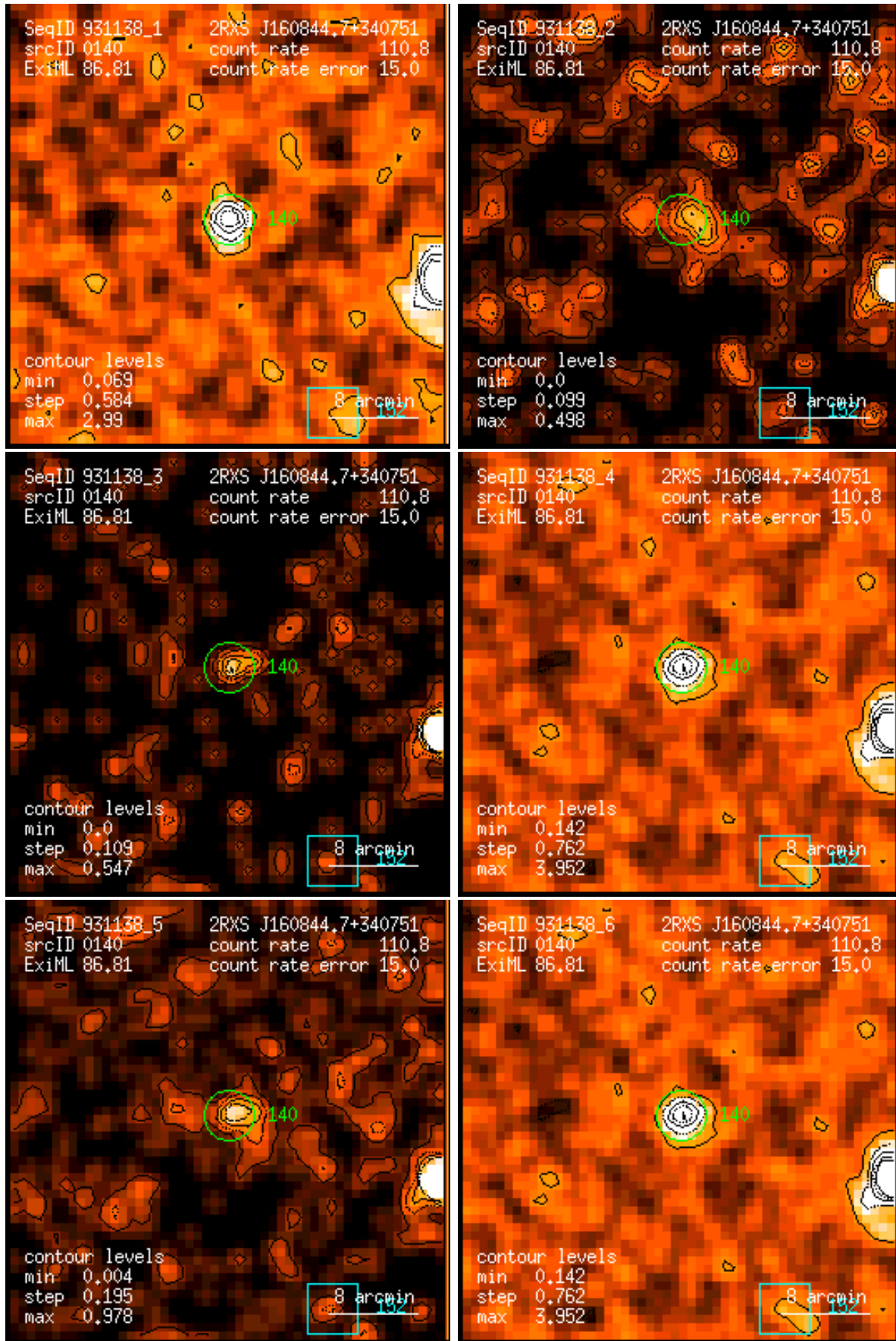
Figure 140: RASS 931138: detection 0140: band rate images, Gaussian filter: (1) PSPC channels 11 – 41, (2) 52 – 90, (3) 91 – 201, (4) 11 – 235, (5) 52 – 201, (6) 11 – 201. Broad band rates in counts/ks. Band rate contour levels in counts/ks/arcmin 2 .
