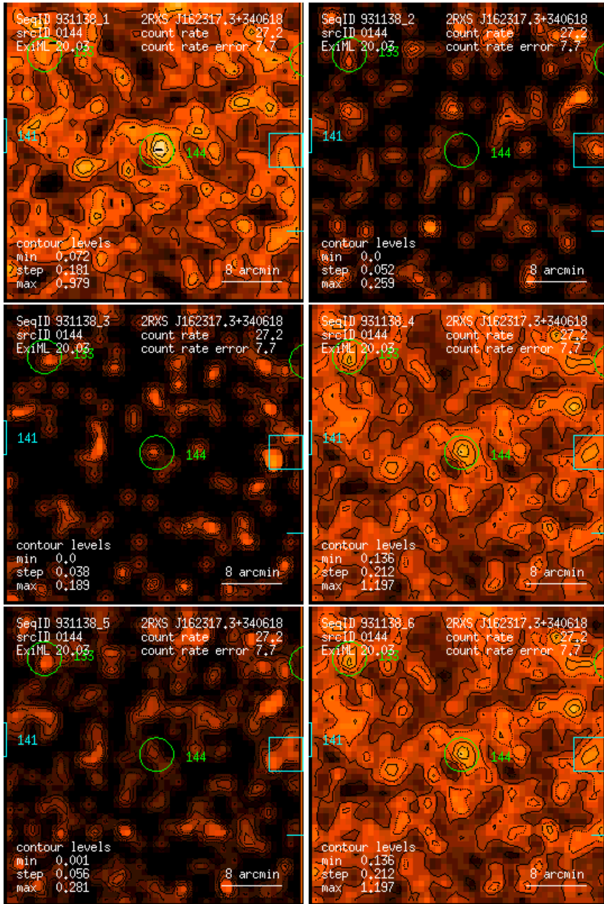
Figure 144: RASS 931138: detection 0144: band rate images, Gaussian filter: (1) PSPC channels 11 – 41, (2) 52 – 90, (3) 91 – 201, (4) 11 – 235, (5) 52 – 201, (6) 11 – 201. Broad band rates in counts/ks. Band rate contour levels in counts/ks/arcmin 2 .
