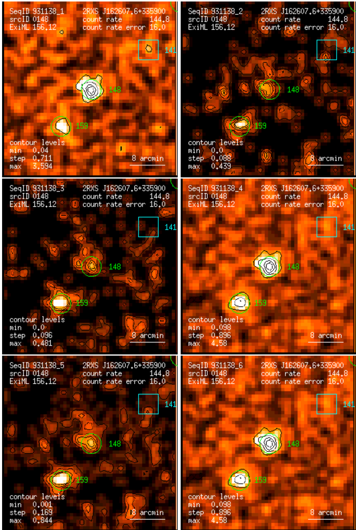
Figure 148: RASS 931138: detection 0148: band rate images, Gaussian filter: (1) PSPC channels 11 – 41, (2) 52 – 90, (3) 91 – 201, (4) 11 – 235, (5) 52 – 201, (6) 11 – 201. Broad band rates in counts/ks. Band rate contour levels in counts/ks/arcmin 2 .
