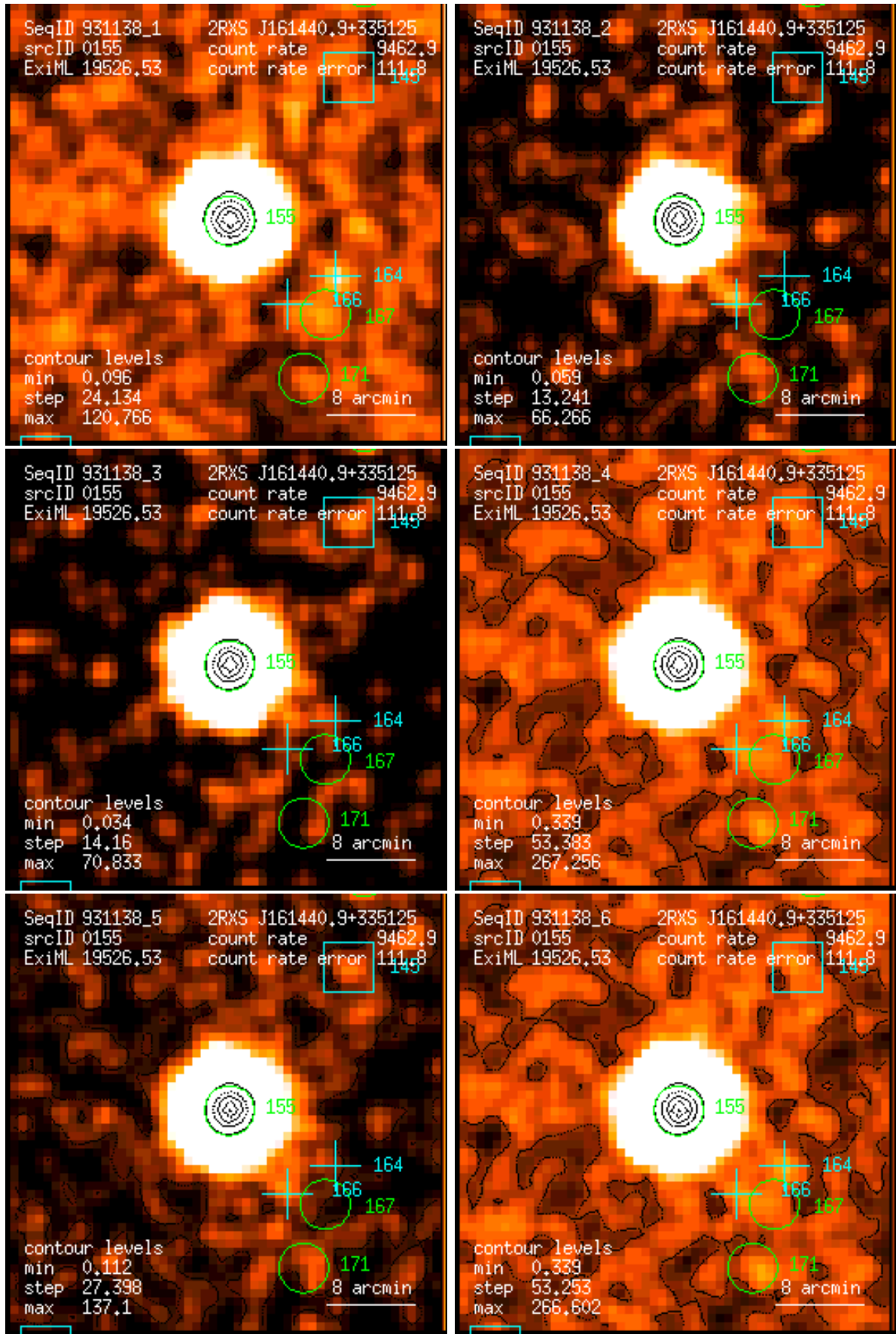
Figure 155: RASS 931138: detection 0155: band rate images, Gaussian filter: (1) PSPC channels 11 – 41, (2) 52 – 90, (3) 91 – 201, (4) 11 – 235, (5) 52 – 201, (6) 11 – 201. Broad band rates in counts/ks. Band rate contour levels in counts/ks/arcmin 2 .
